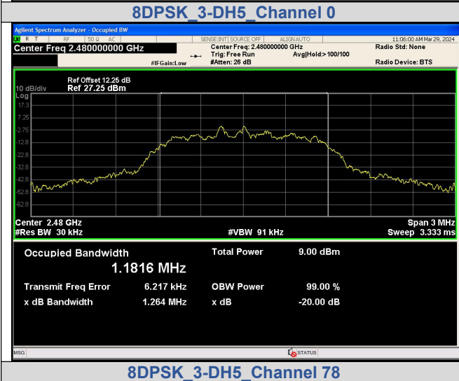
8DPSK 3-DH5 Channel 78
