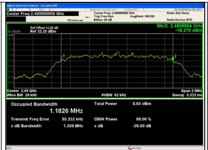
\pi/4 DQPSK_2-DH5_Channel 78
