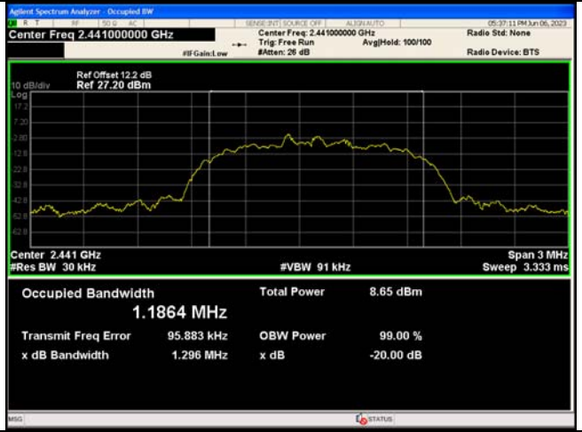
8DPSK_3-DH5_Channel 39
