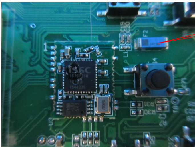
BT Antenna
