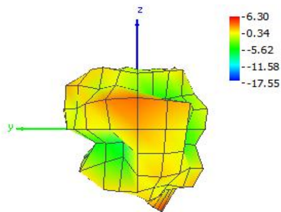
2500MHz, Max PK Gain=6.30dBi
