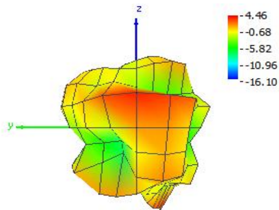
2450MHz, Max PK Gain=4.46dBi
