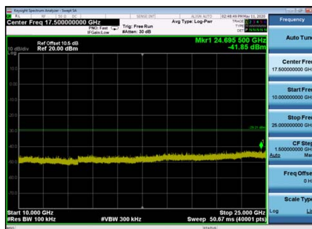
,Plot ,5Transmitter Spurious Emission : 2440,10000MHz~25000MHz
