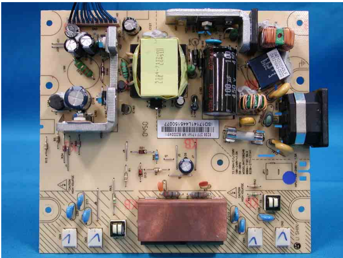
PCB Layout (LI-Shin Power)
