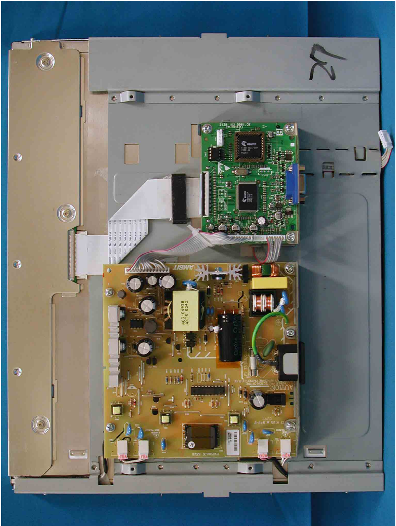
Assembly w/o Shielding
