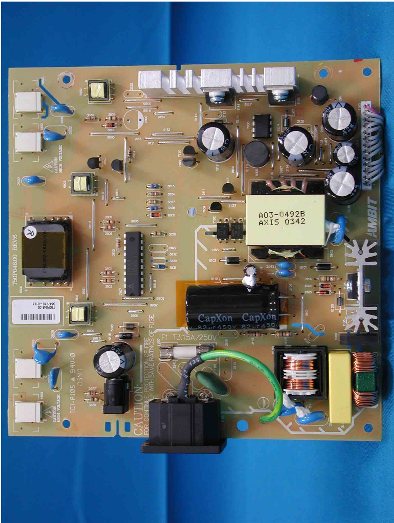
PCB Layout (Ambit Power)
