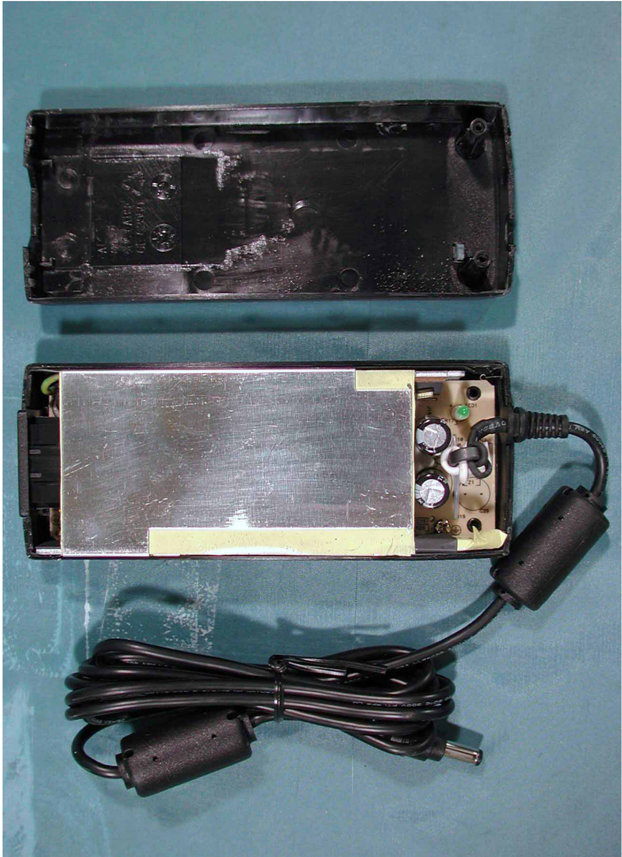
Adapter Assembly
