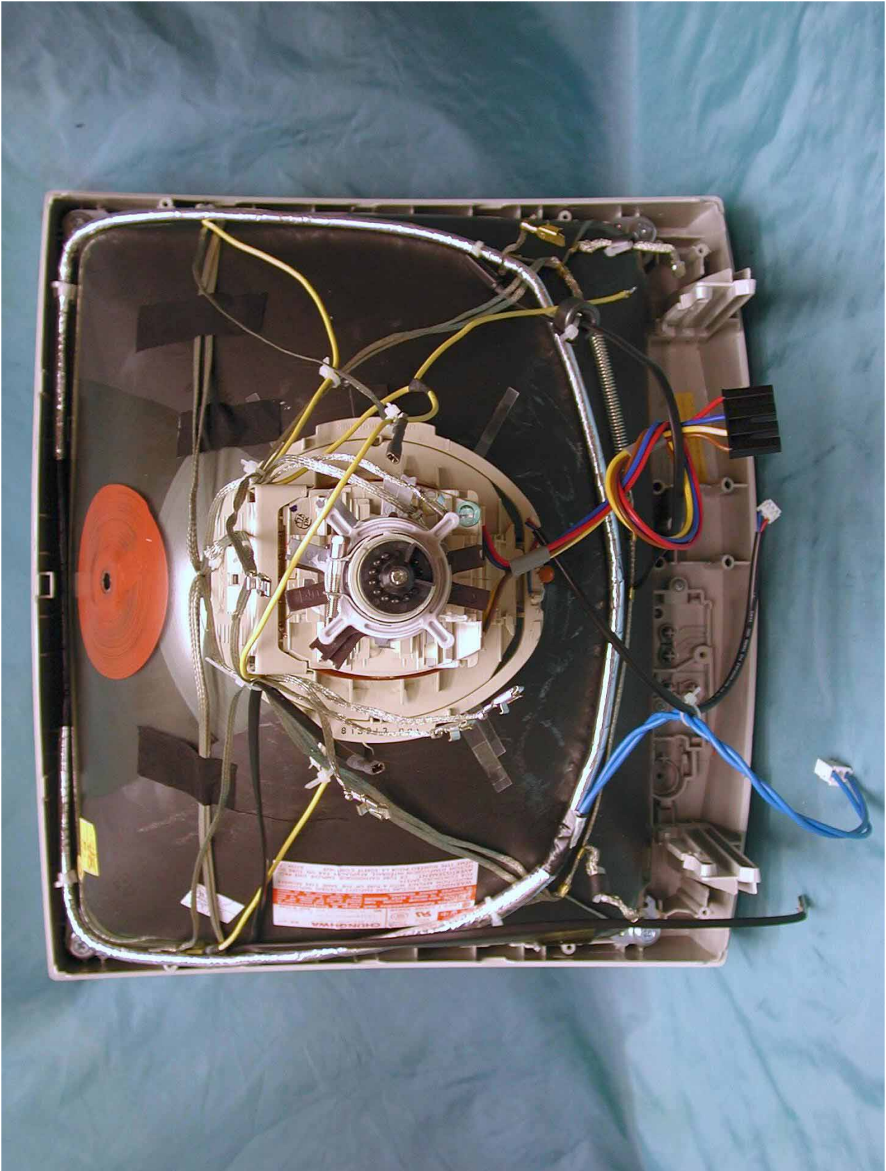
CRT Assembly
