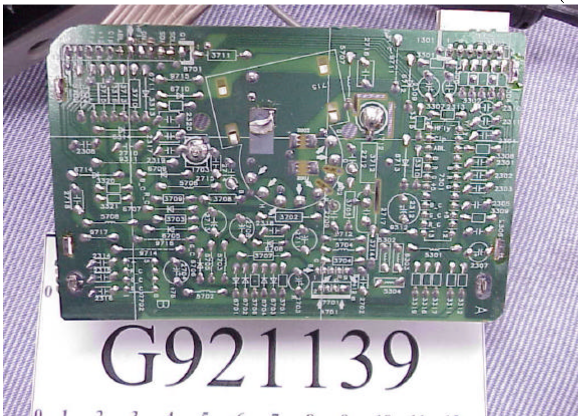
Figure 12 Display Color Monitor Video Board (Foil Side)
