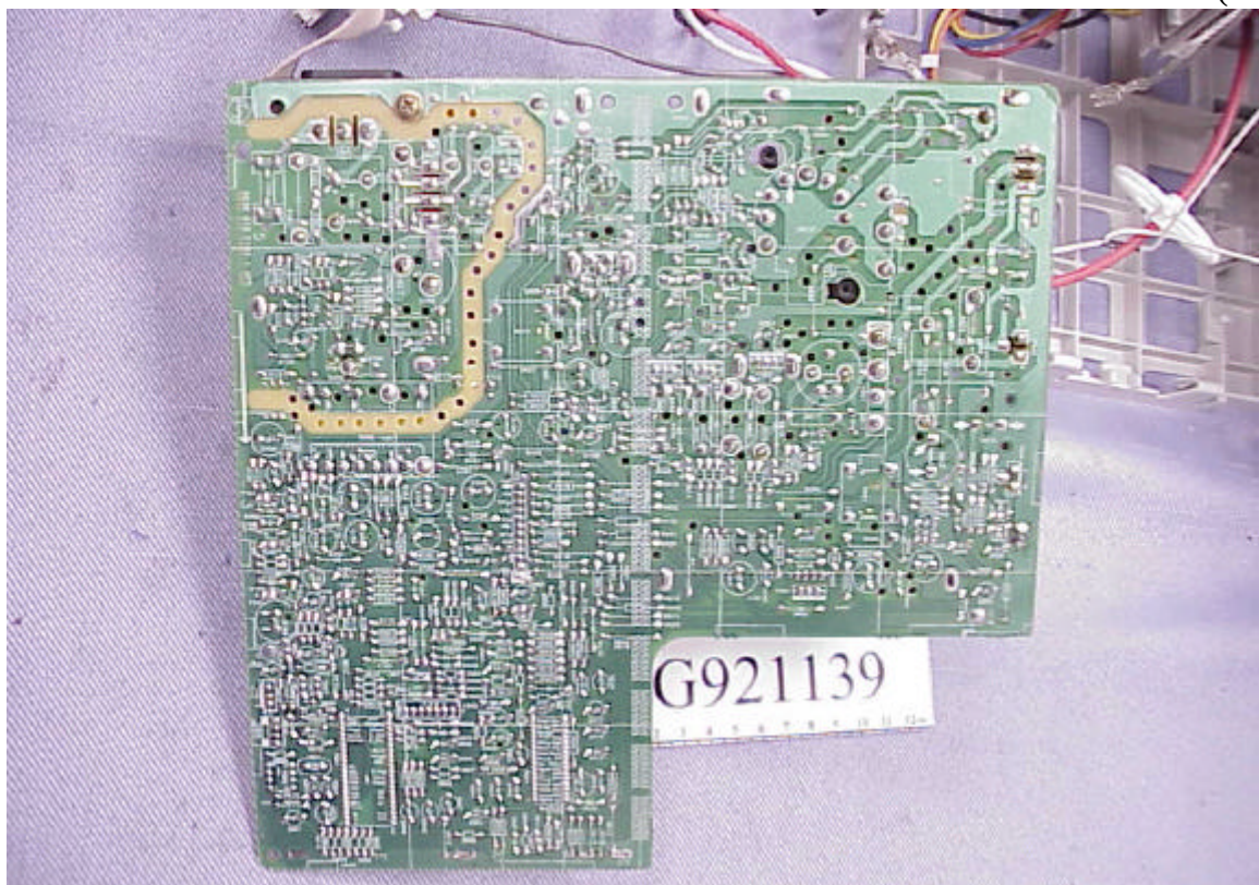
Figure 14 Display Color Monitor Main Board (Foil Side)
