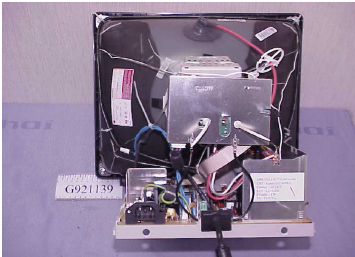
Figure 7 Display Color Monitor Internal View
