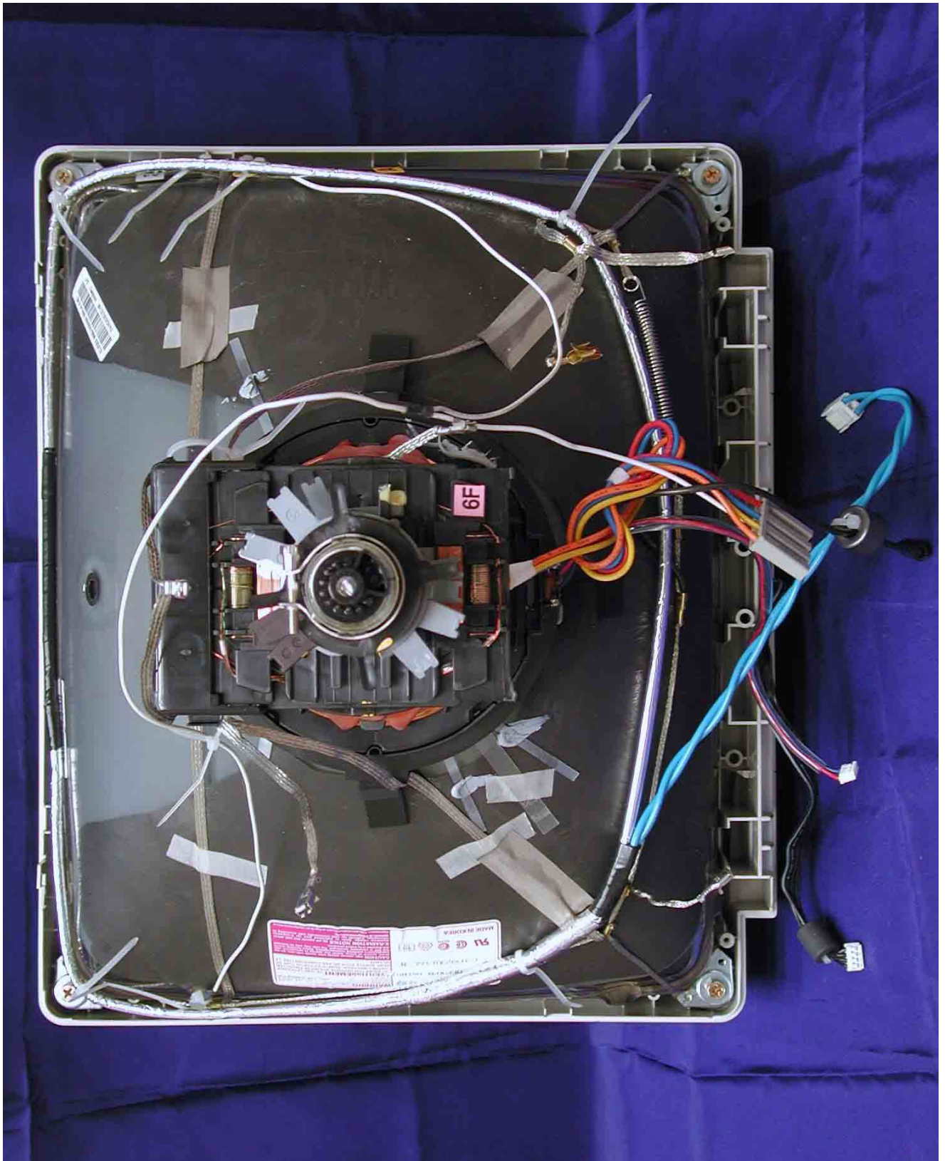
CRT Assembly
