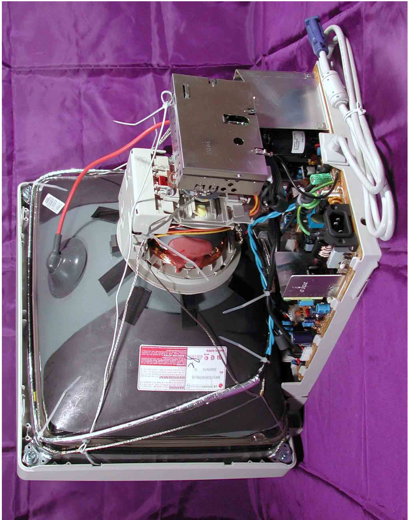
Side View Without Back Cover
