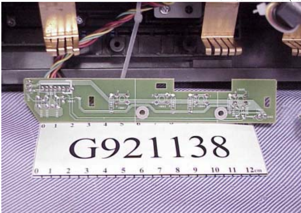
Figure 26 Display Color Monitor Front Control Board (Foil View)
