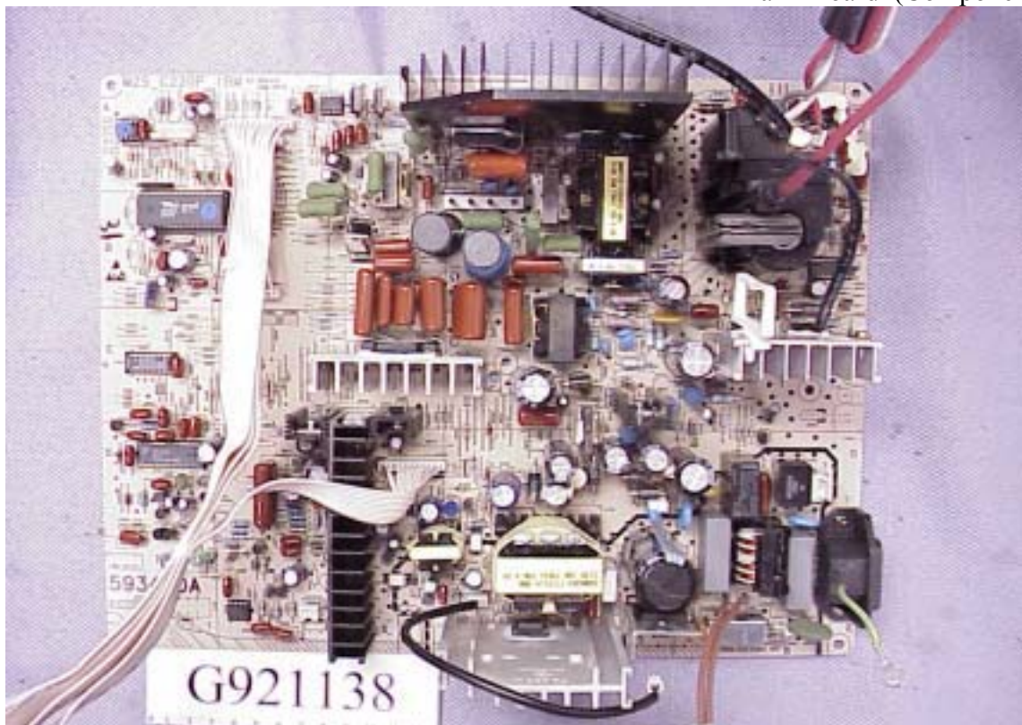
Figure 24 Display Color Monitor Main Board (Component View)
