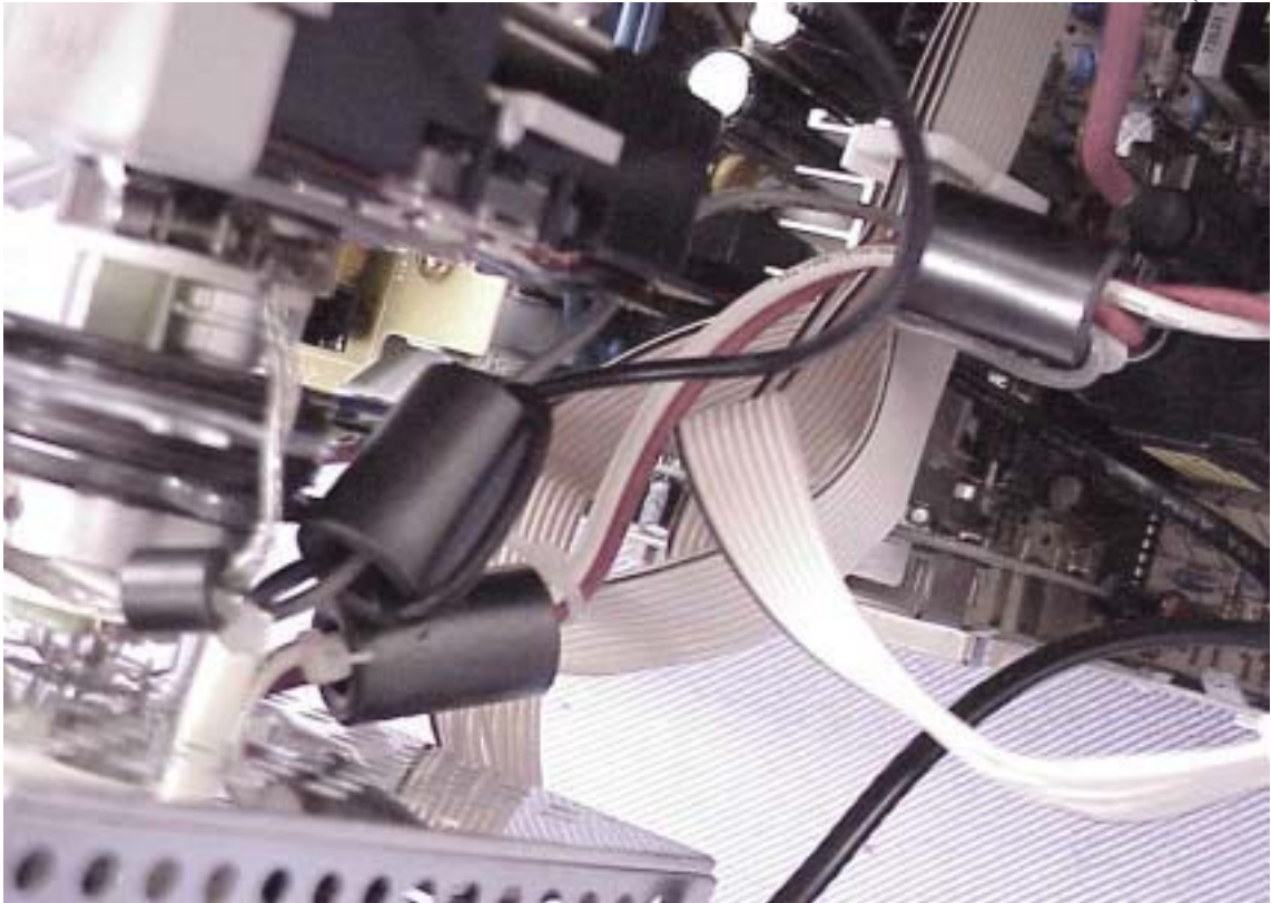
Figure 11 Display Color Monitor Internal View (Ferrite Core)
