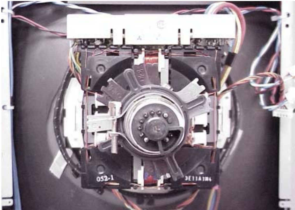
Figure 13 Display Color Monitor Frame of CRT
