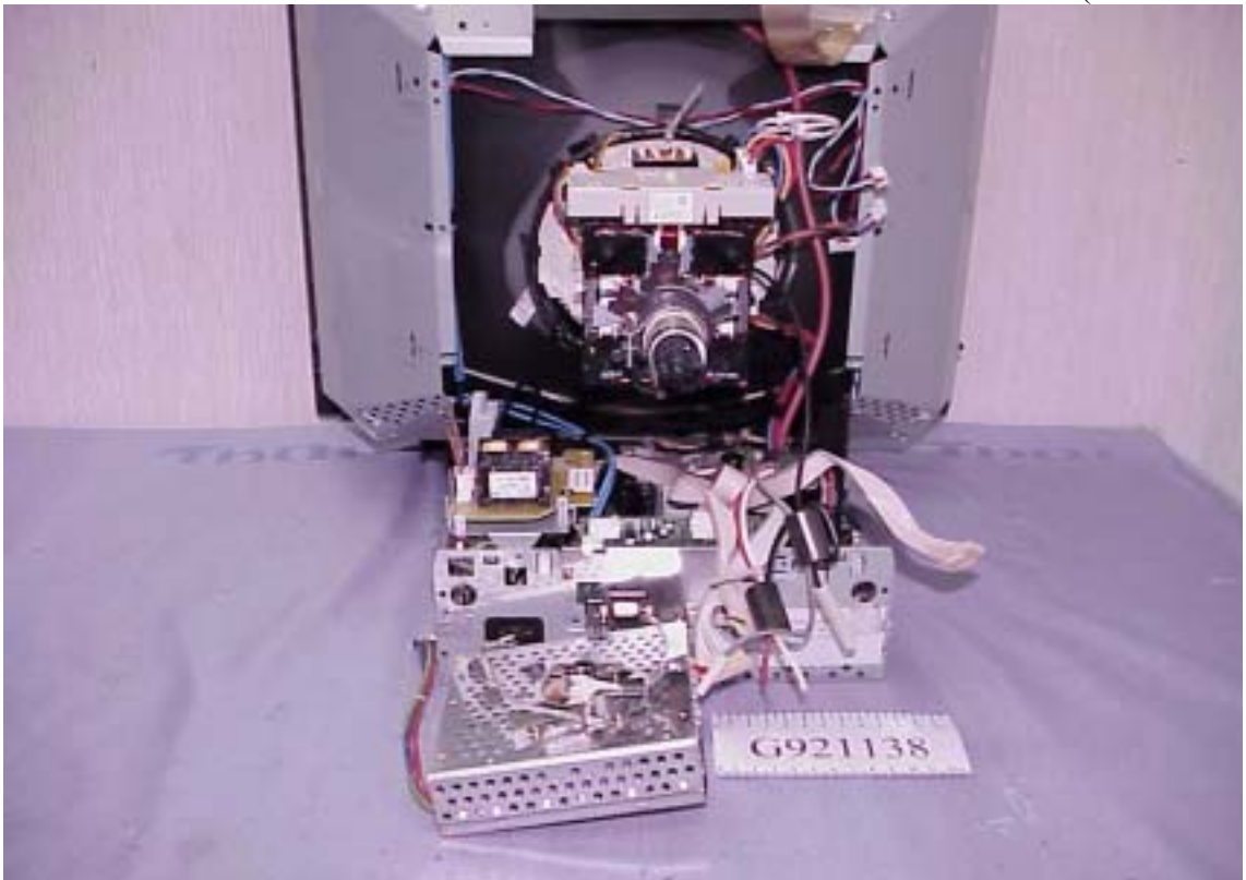
Figure 12 Display Color Monitor Removed the Video Board (Frame of Internal)
