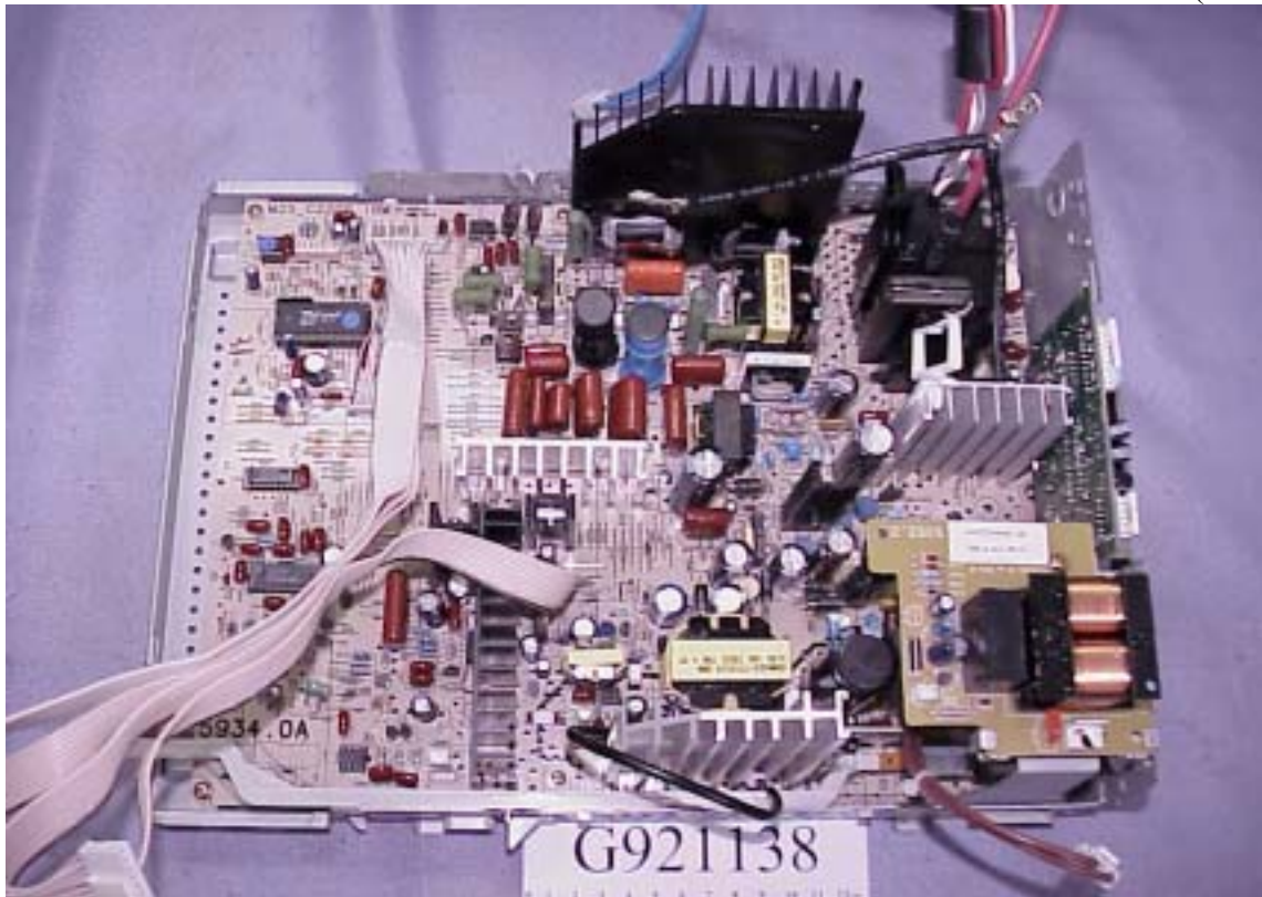
Figure 19 Display Color Monitor Main Board (Front View)
