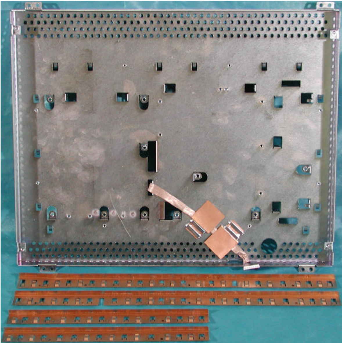
Shielding Plate
