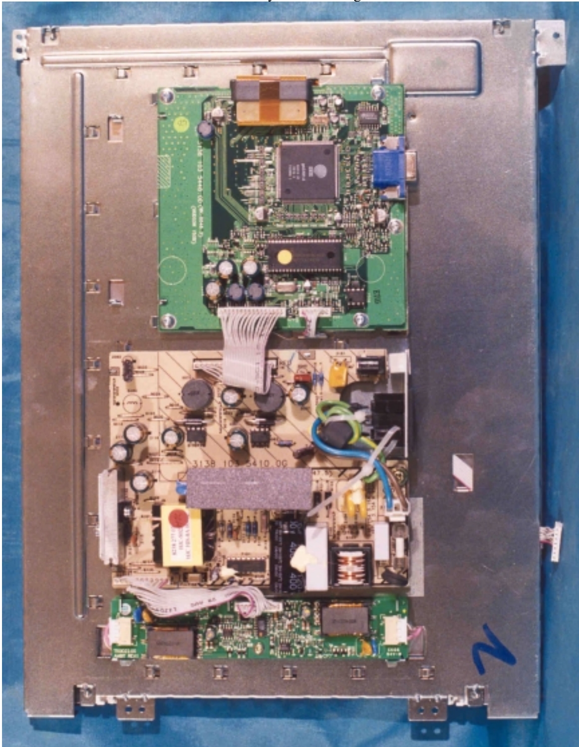
Panel Assembly w/o Shielding Cover
