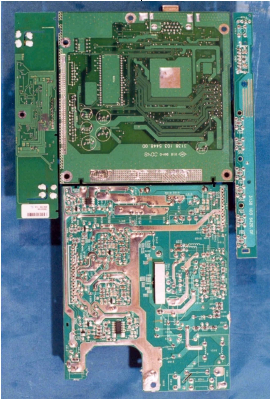
PCB Layout
