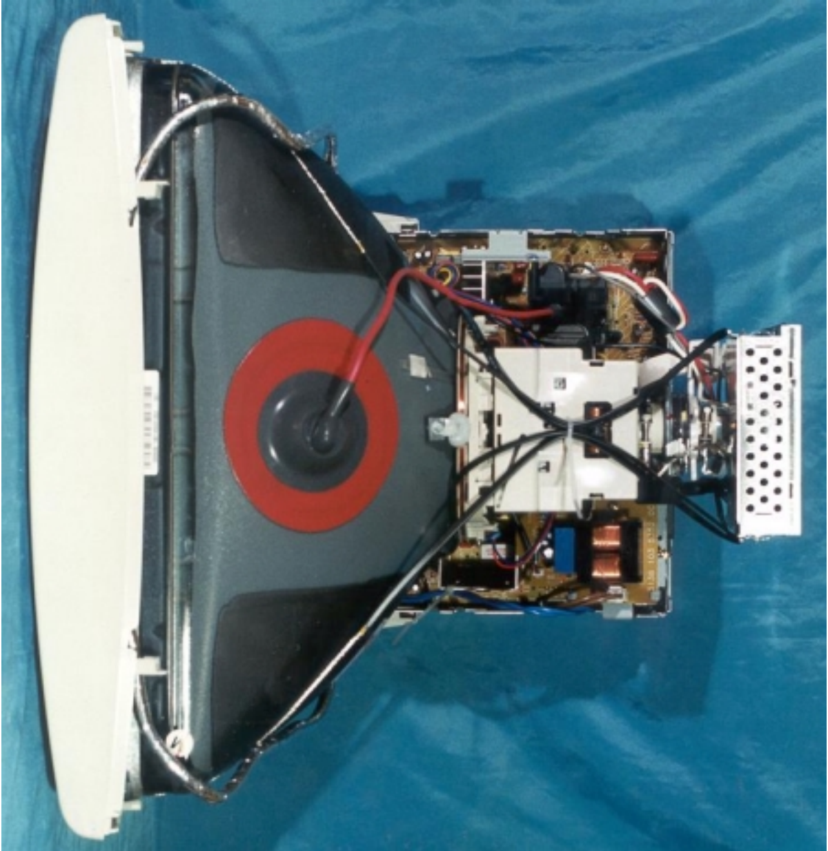
Top View w/o Shielding Cover
