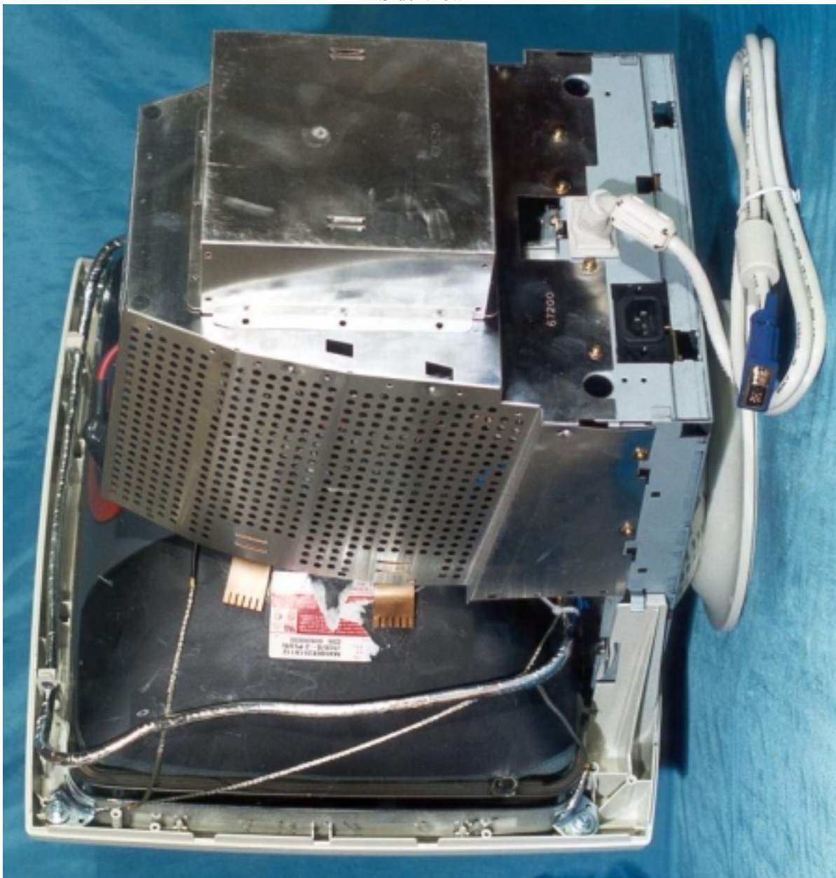
Side View
