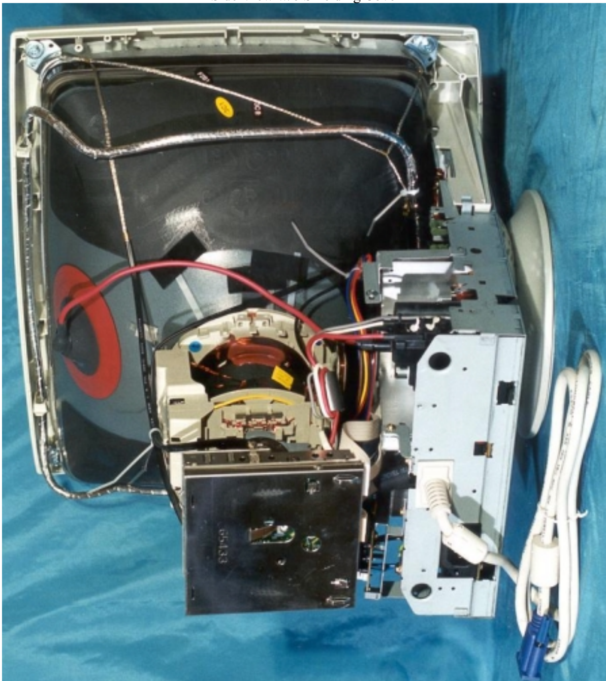
Side View w/o Shielding Cover
