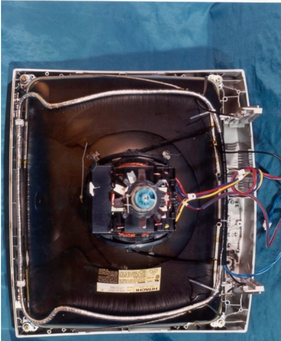
CRT Assembly
