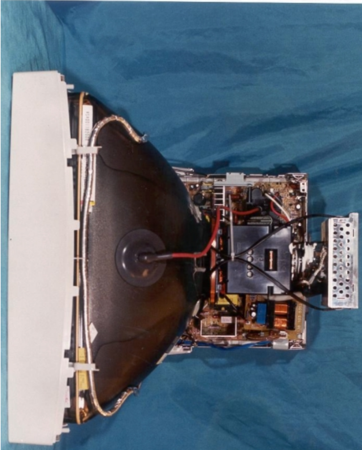
Top View w/o Shielding Cover
