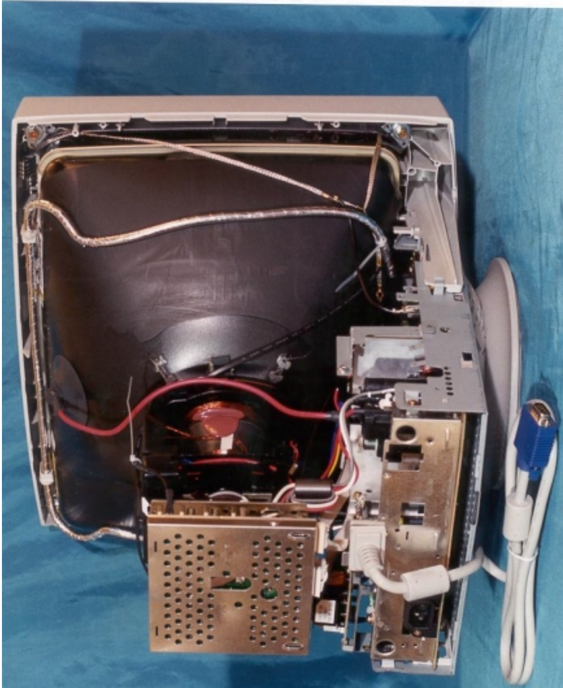
Side View w/o Shielding Cover
