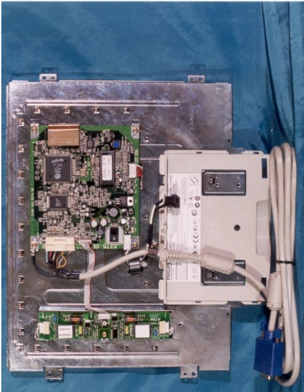
Rear view w/o Shielding Cover
