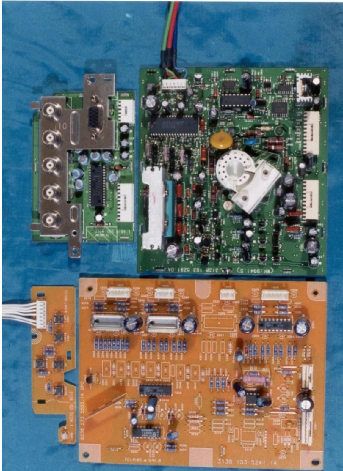
PCB Layout
