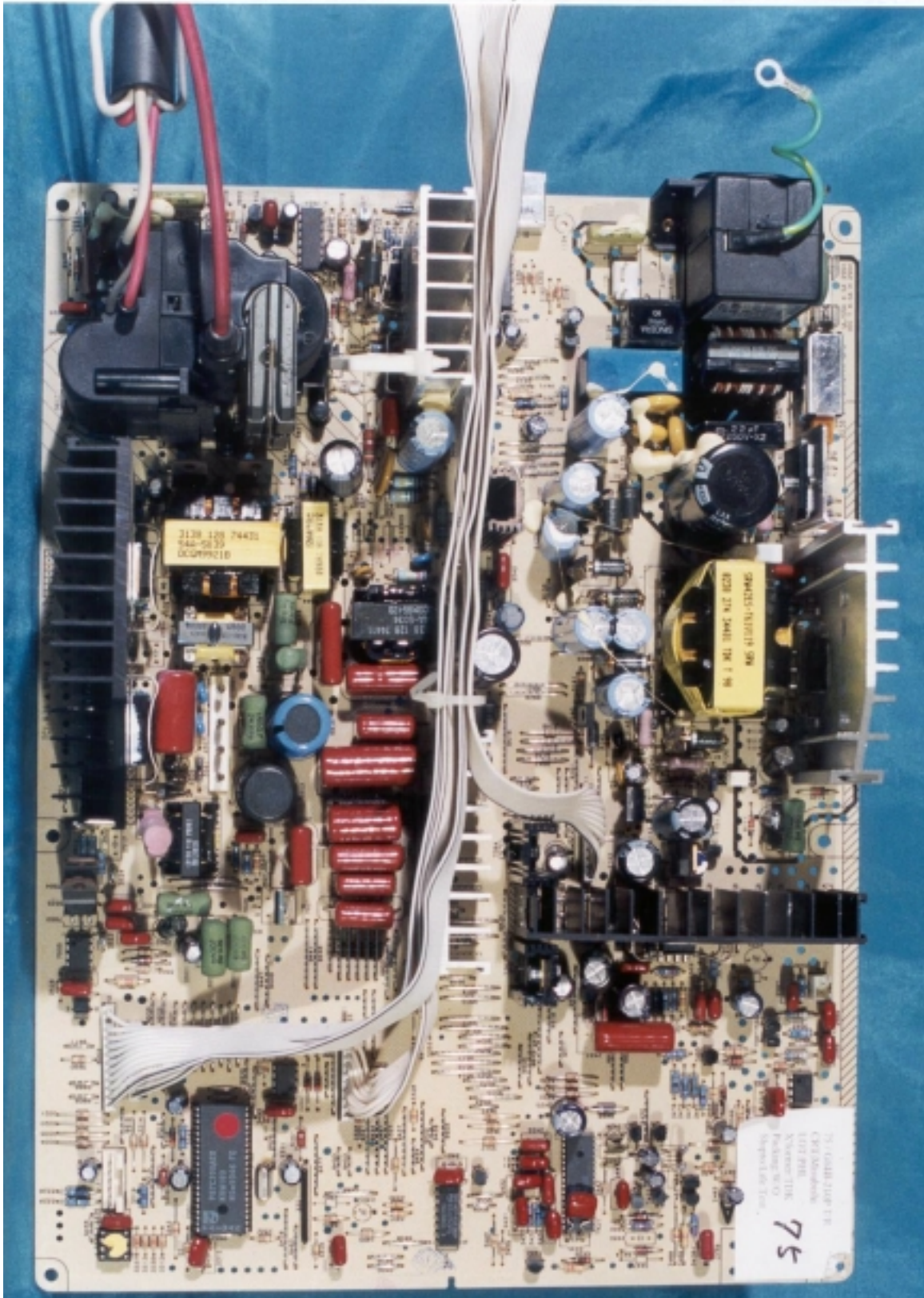
PCB Layout
