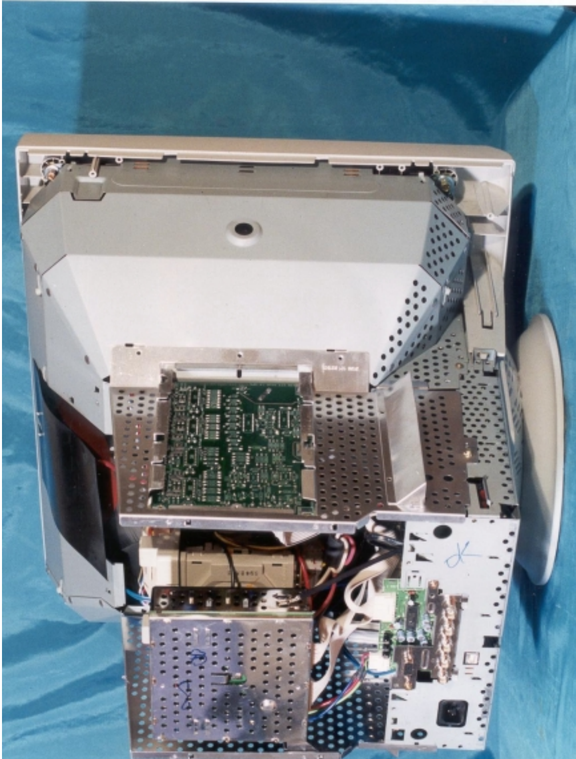
Side View w/o Shielding Cover
