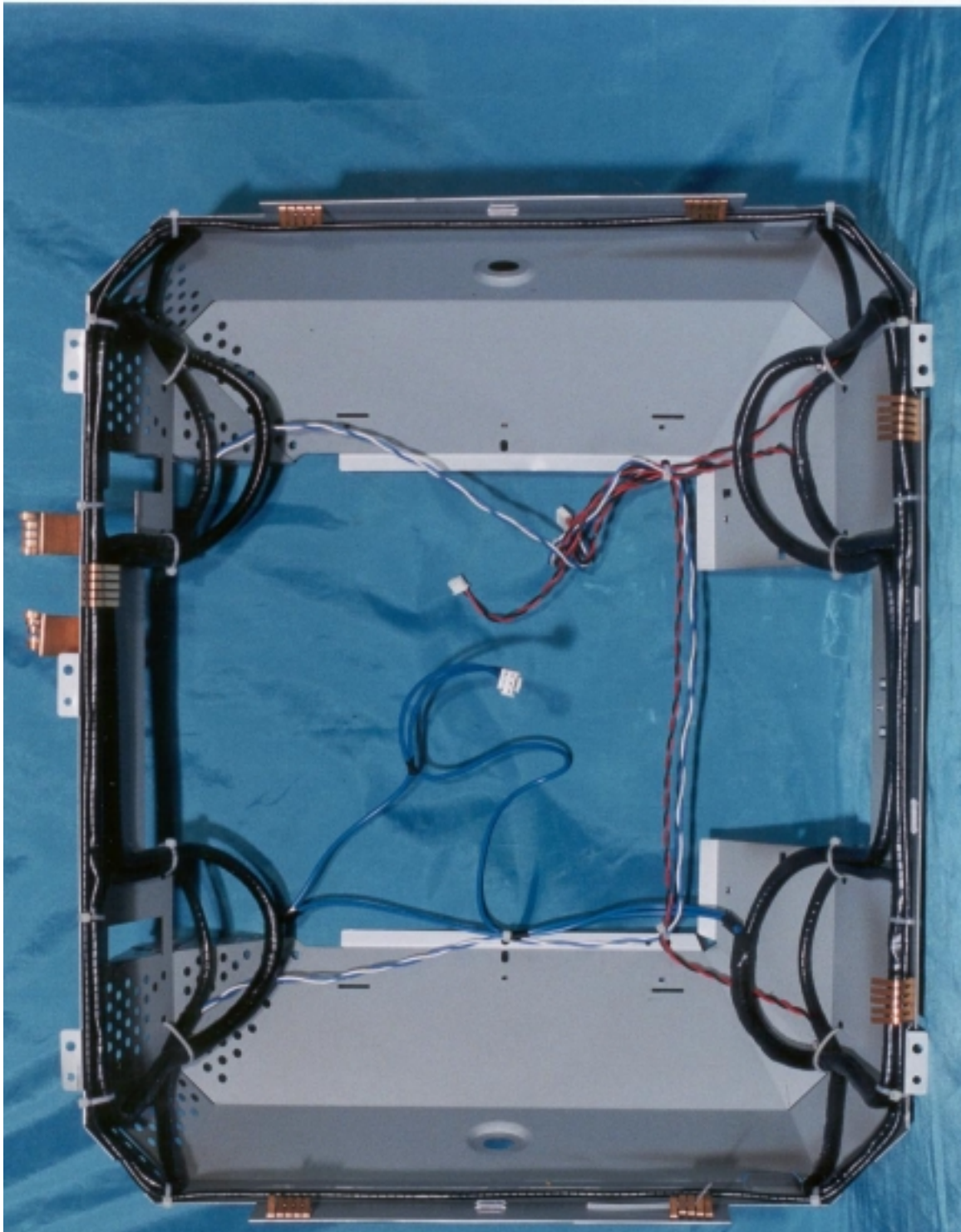
Shielding frame
