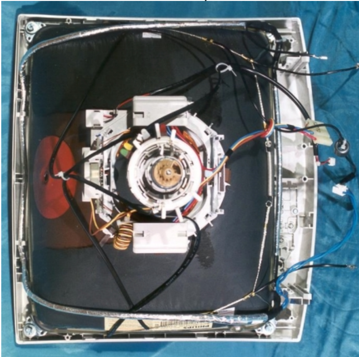
CRT Assembly
