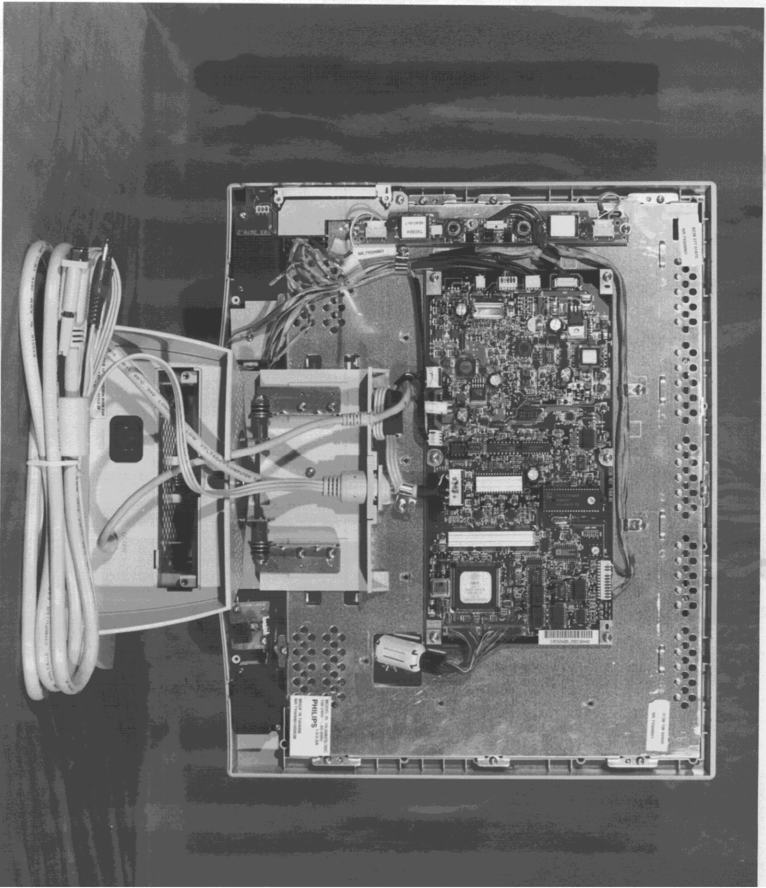
Rear View w/o Metal Cover
