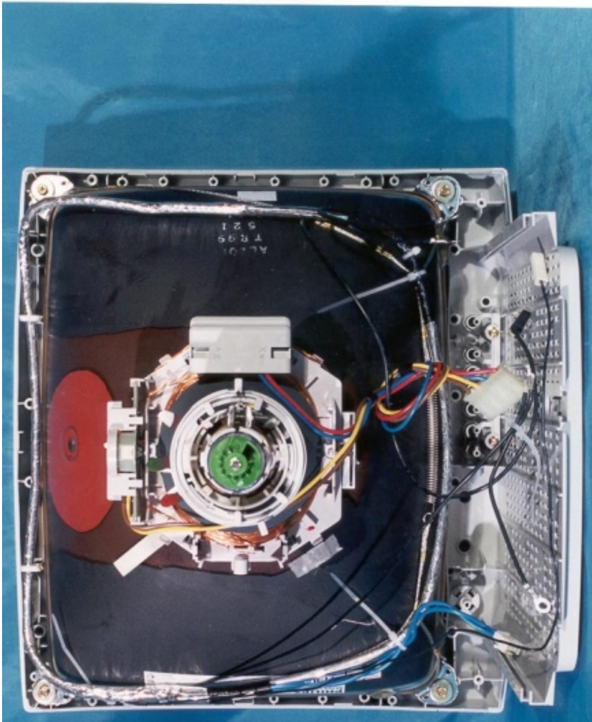
CRT Assembly
