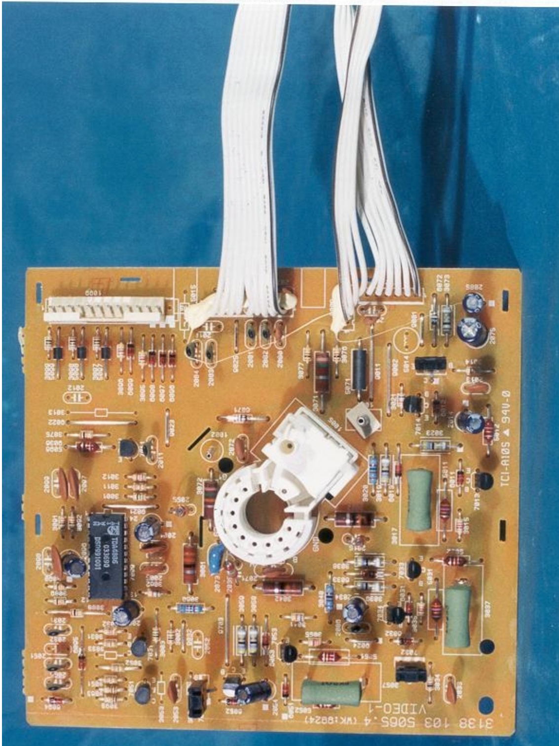
PCB Layout
