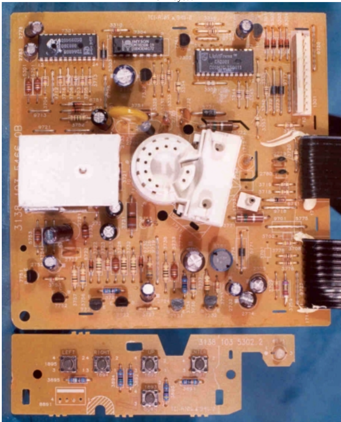
PCB Layout
