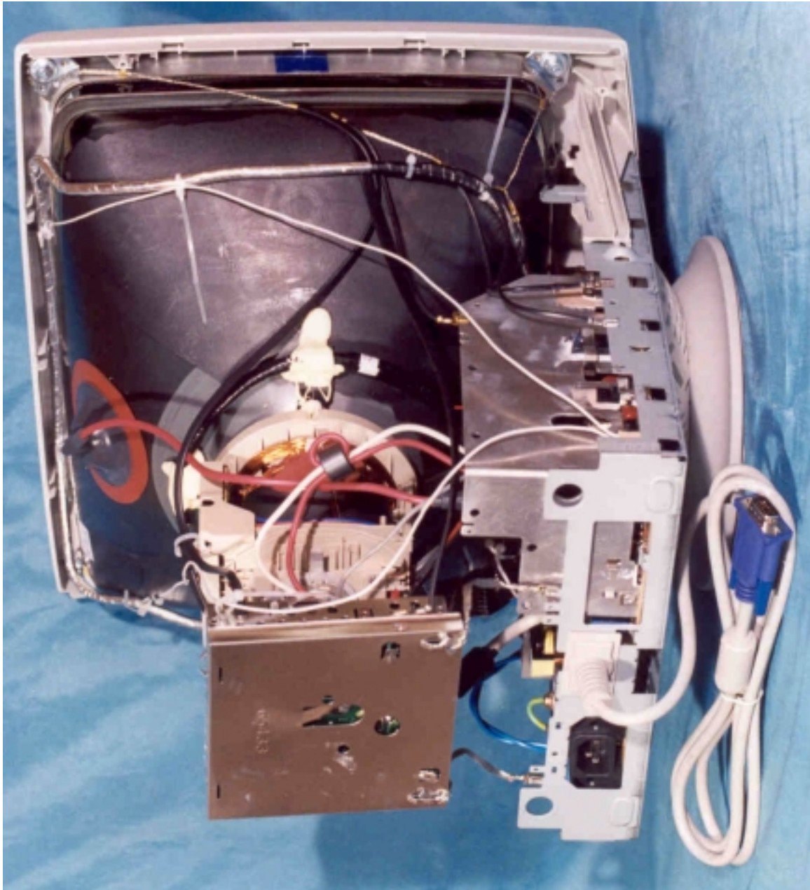
Side View
