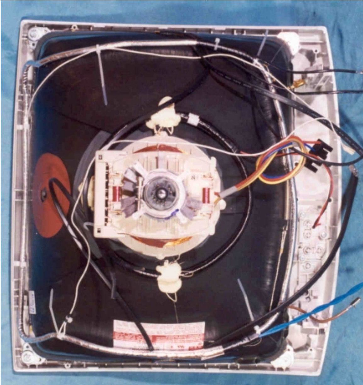
CRT Assembly
