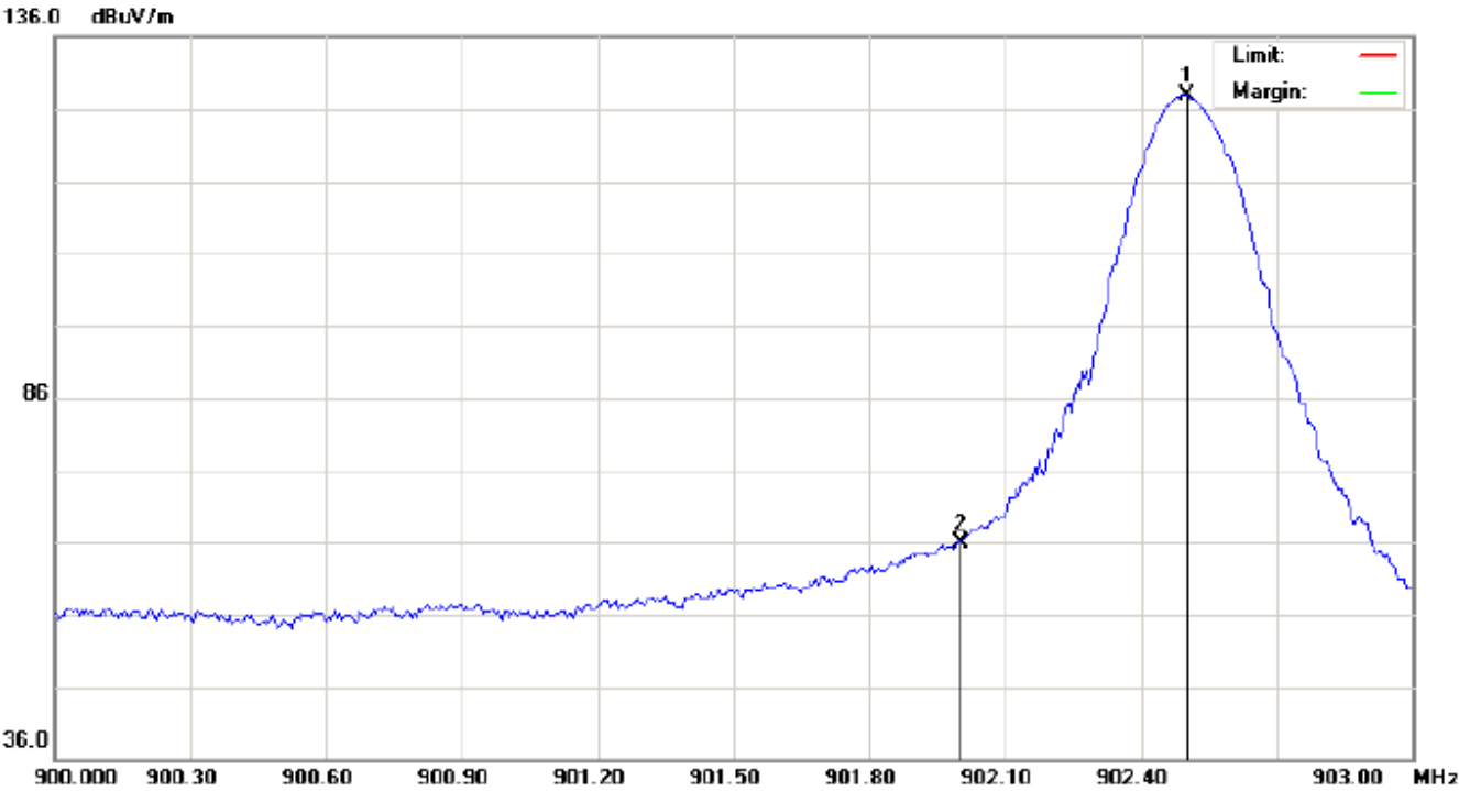
TEST PLOT OF BAND EDGE FOR LOW CHANNEL -H
