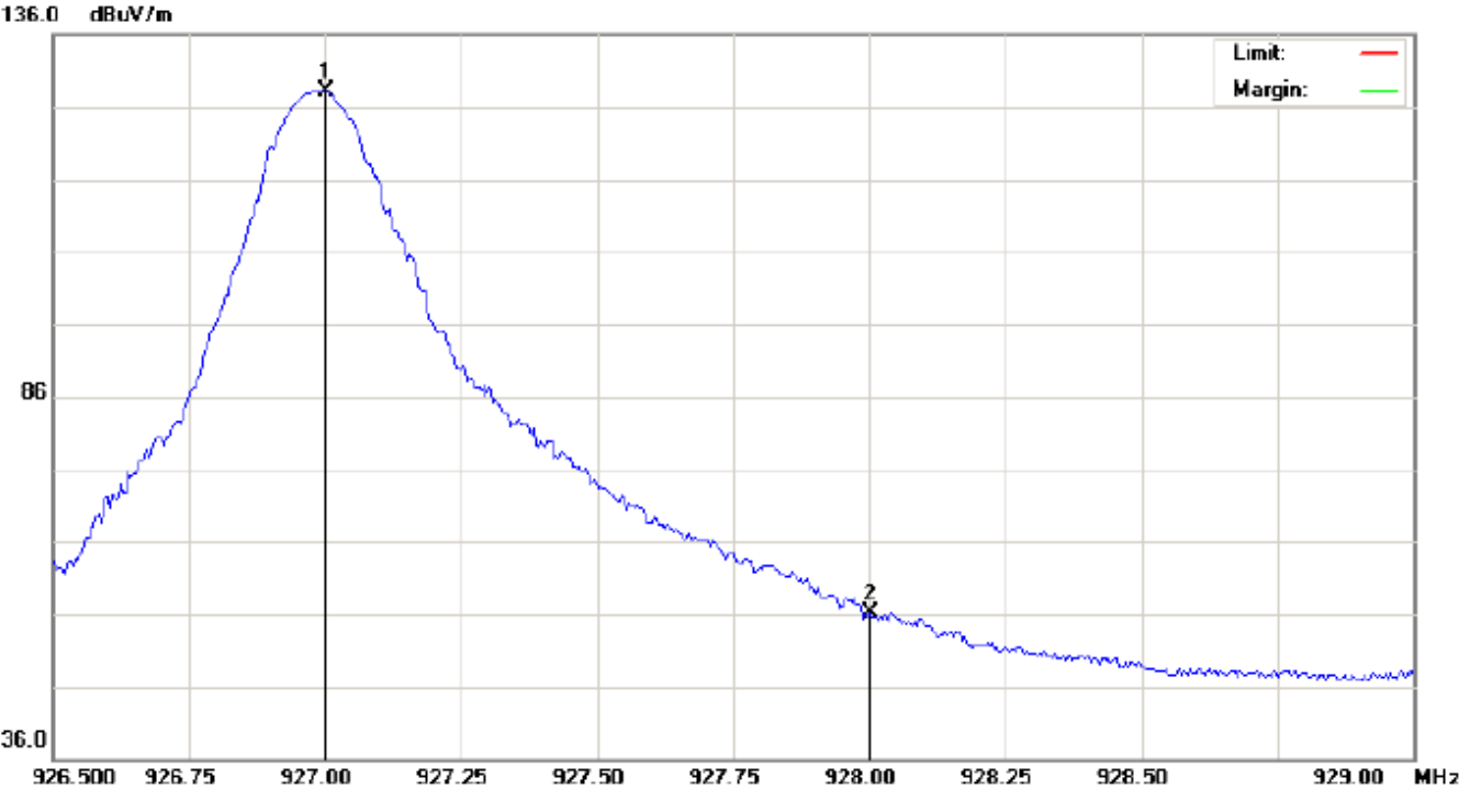
TEST PLOT OF BAND EDGE FOR HIGH CHANNEL-H
