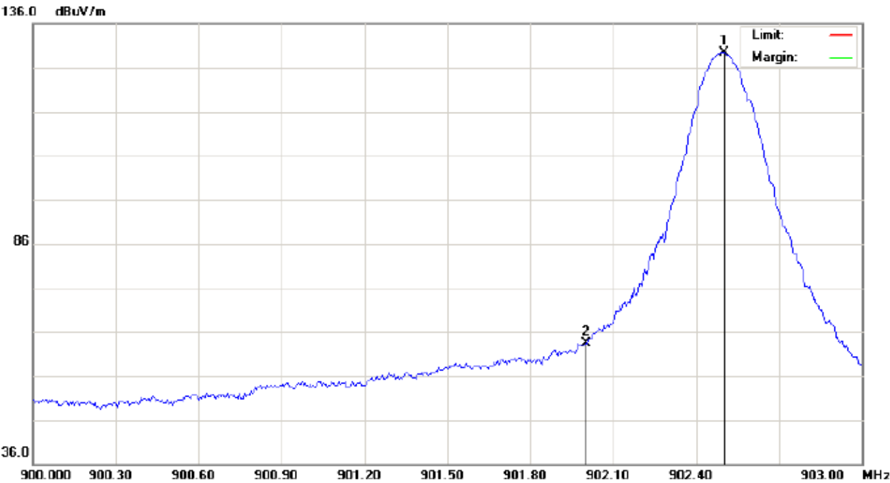
TEST PLOT OF BAND EDGE FOR LOW CHANNEL –V
