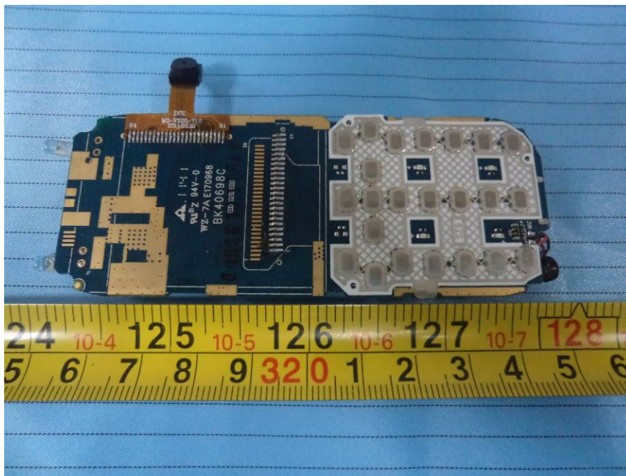
EUT – Main Board Top without LCD View
