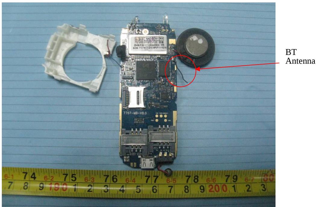
EUT – Antenna Cradle off View 2
