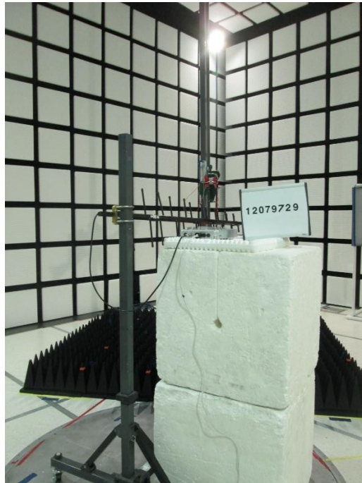
RADIATED BACK UHF LOG PERIODIC ANTENNA
