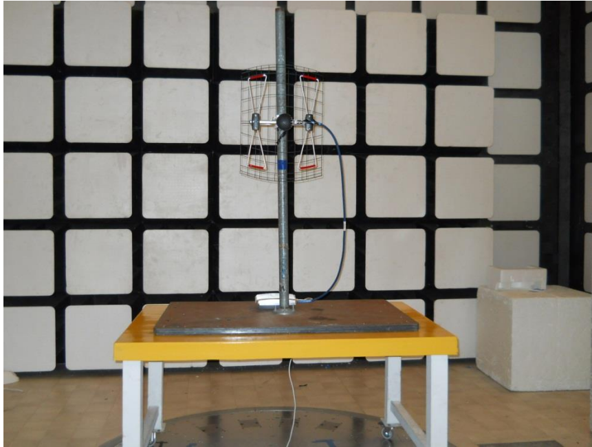
RADIATED FRONT –DB2E ANTENNA
