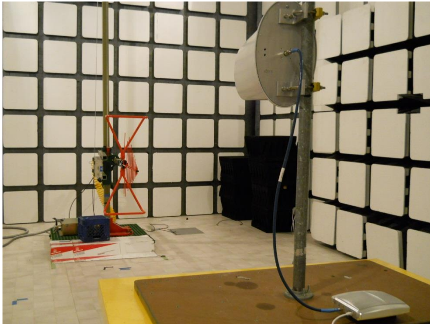
RADIATED BACK –FLAG ANTENNA
