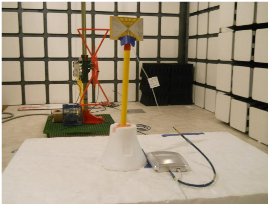
RADIATED BACK –PCB ANTENNA
