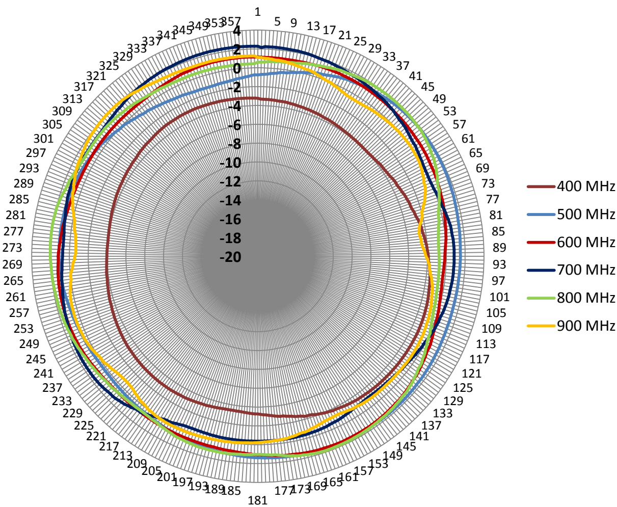
PCB Bowtie Azimuth Pattern
