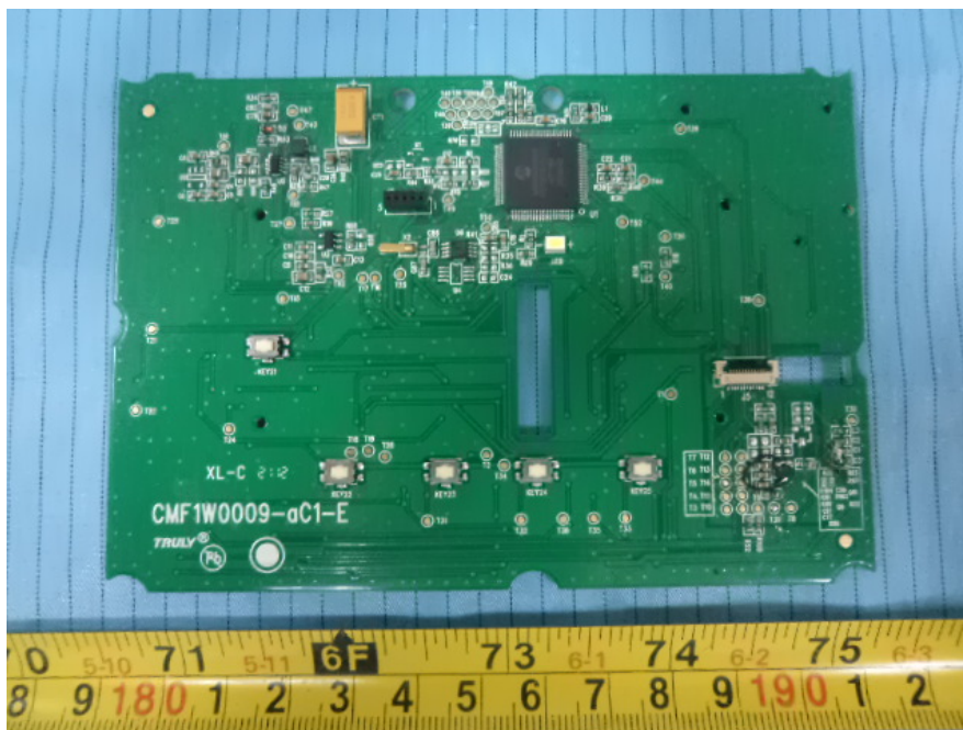
EUT – Main Board Top without RF module View
