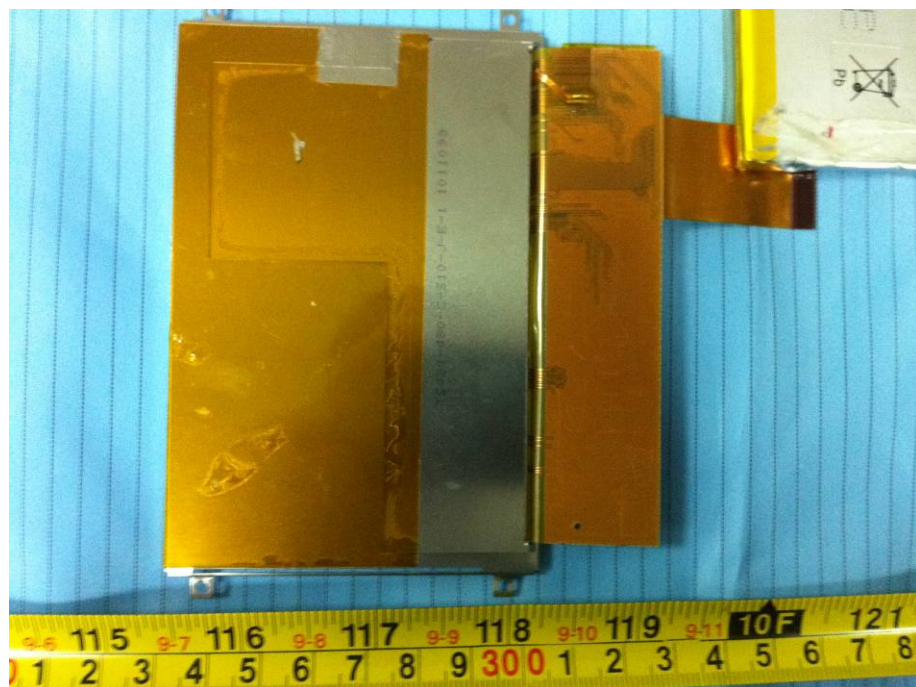
EUT – LCD Display Bottom View
