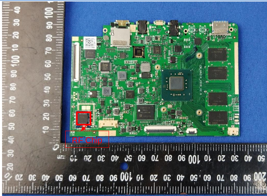
MAIN BOARD TOP VIEW
