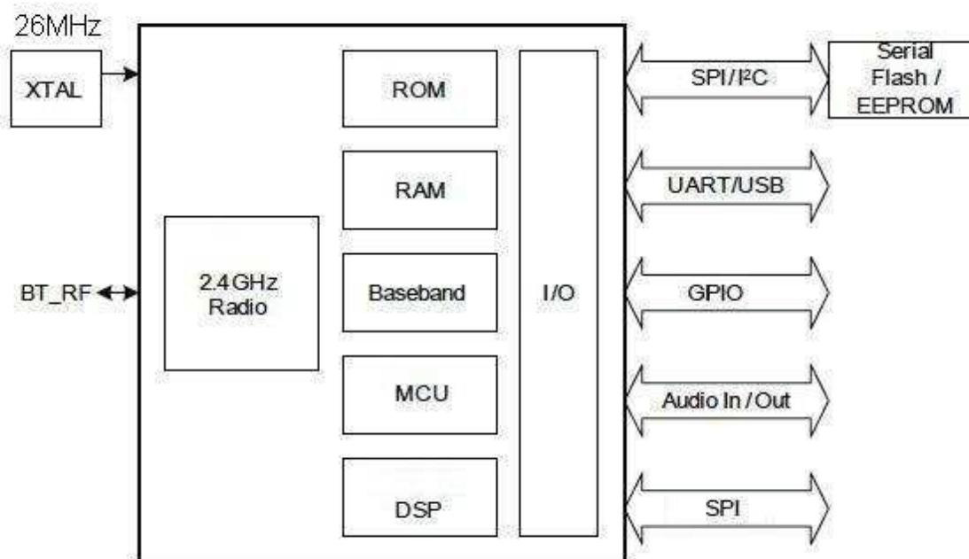
CW6638M Block Diagram
