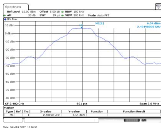
GFSK LOW CHANNEL, CARRIER LEVEL
