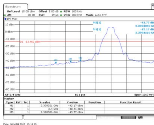
GFSK LOW CHANNEL, BAND EDGE
