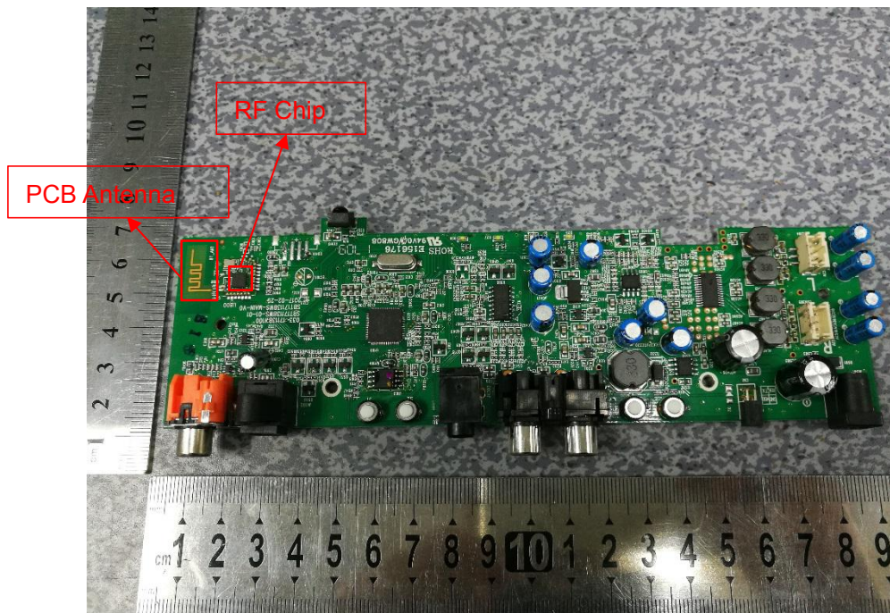
MAIN BOARD TOP VIEW 1 (Soundbar)
