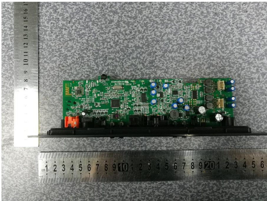
EUT UNCOVER VIEW 2 (Soundbar)
