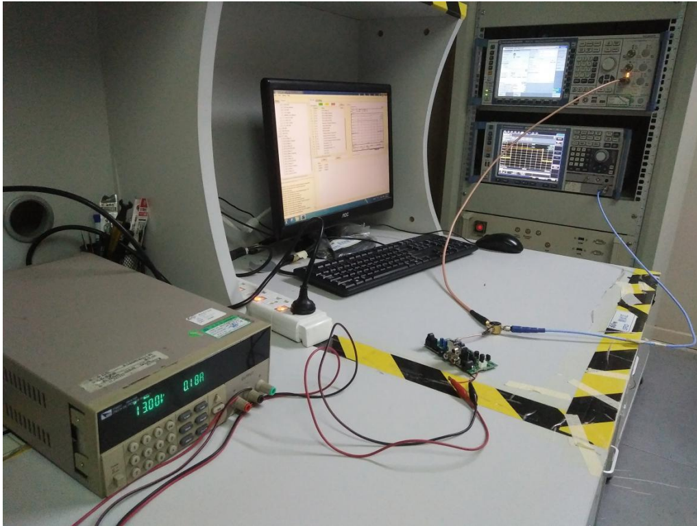
Conducted Test
