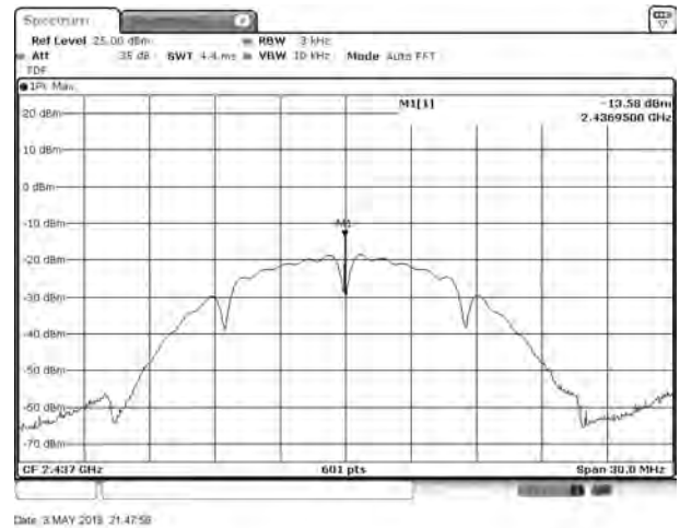
802.11b MIDDLE CHANNEL
