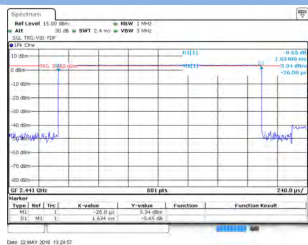
GFSK DH3
