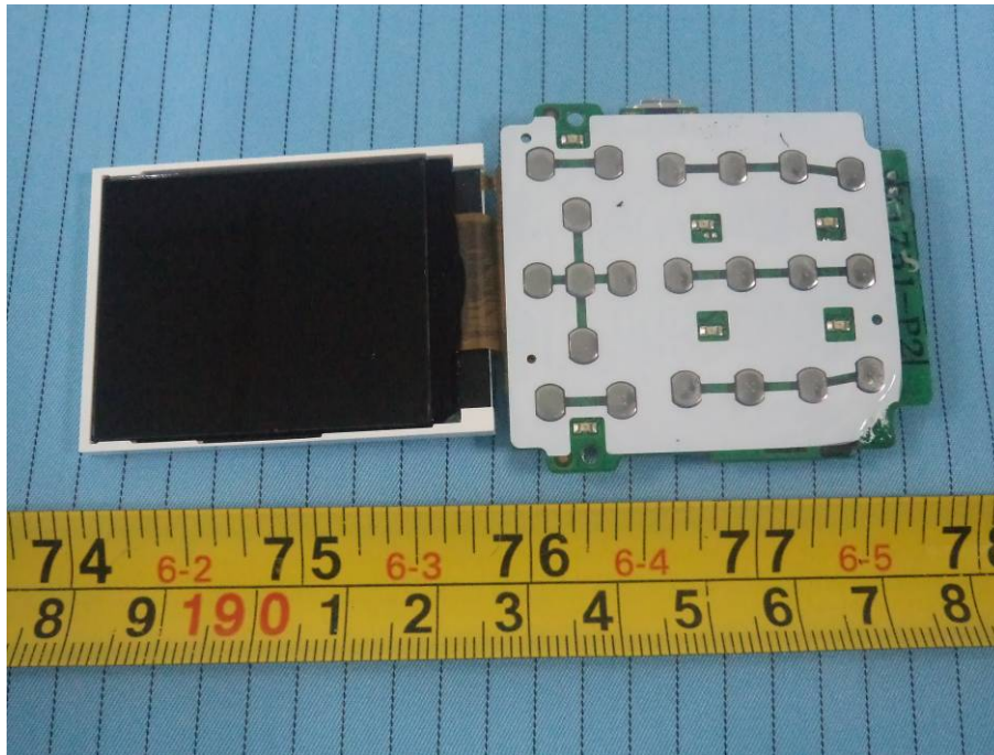
EUT – Main Board Bottom & LCD View1
