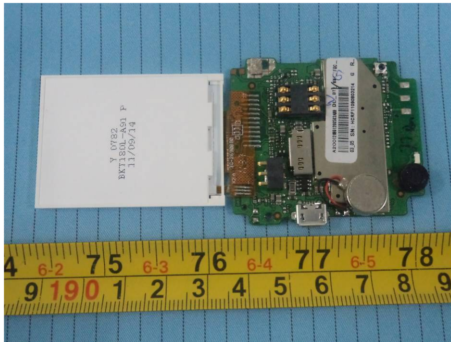
EUT – Main Board Top & LCD View
