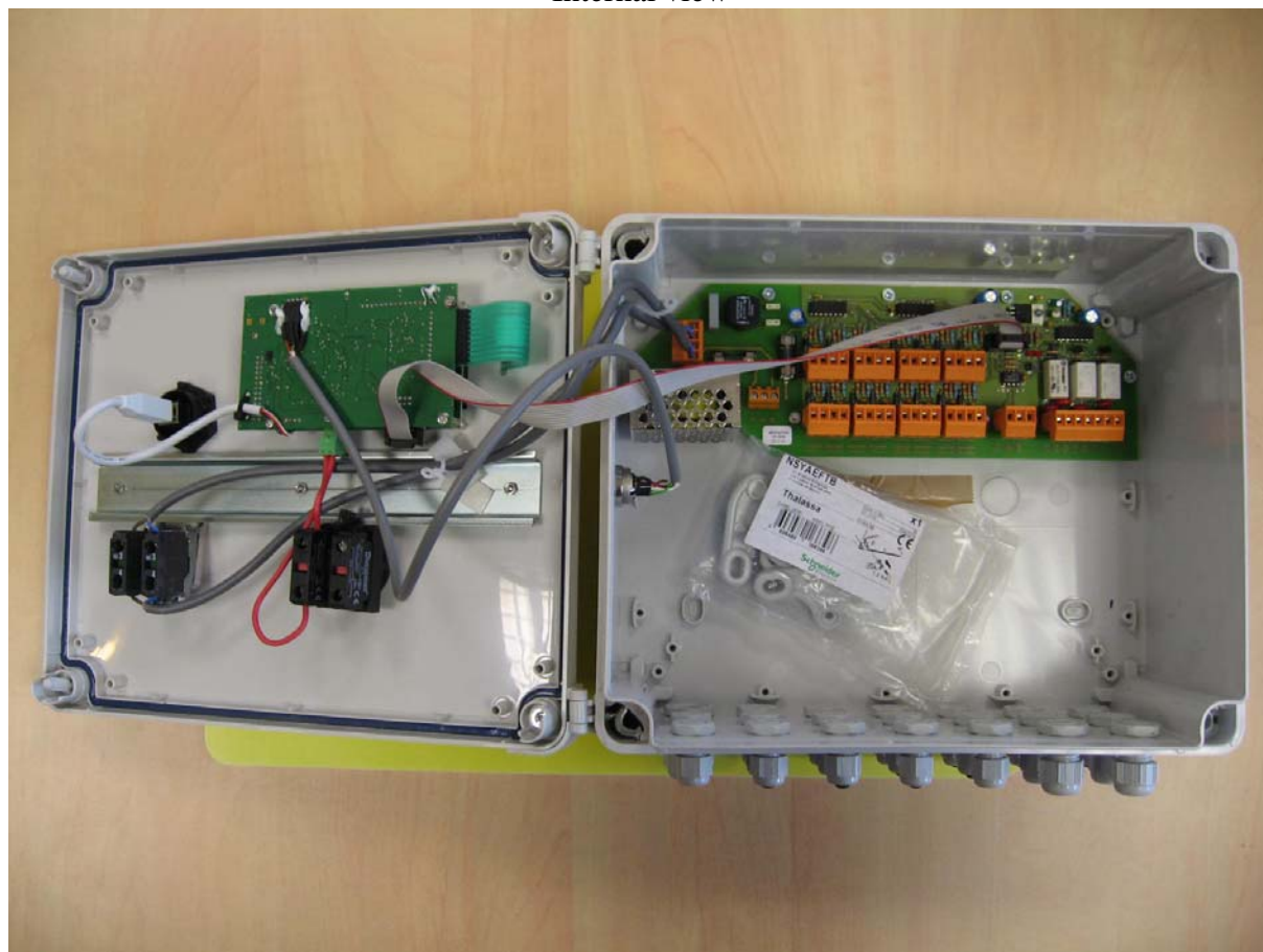
Internal view
