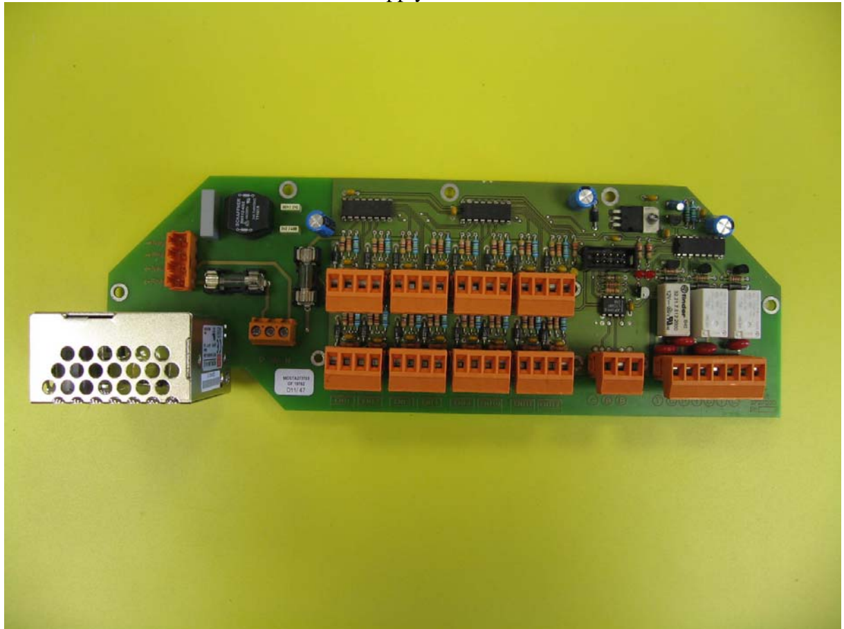
Supply board
