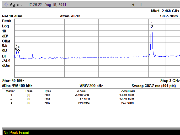
(Plot C.3: Channel = 11, 30MHz to 3GHz)
