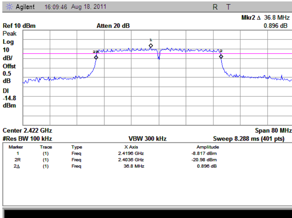
(Plot J: Channel 3: 2422MHz @ 802.11n)
