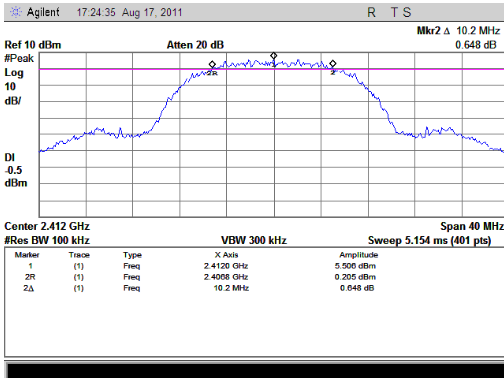
(Plot A1: Channel 1: 2412MHz @ 802.11b)
