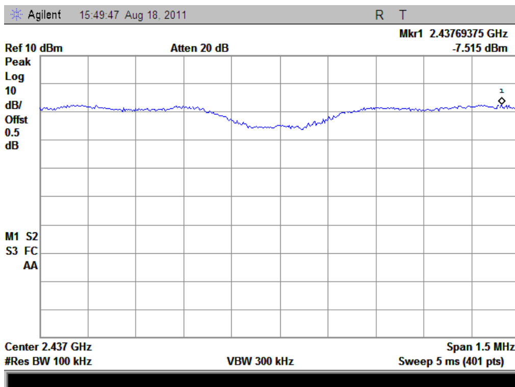
(Plot E.1: Channel = 6 @ 802.11g)
