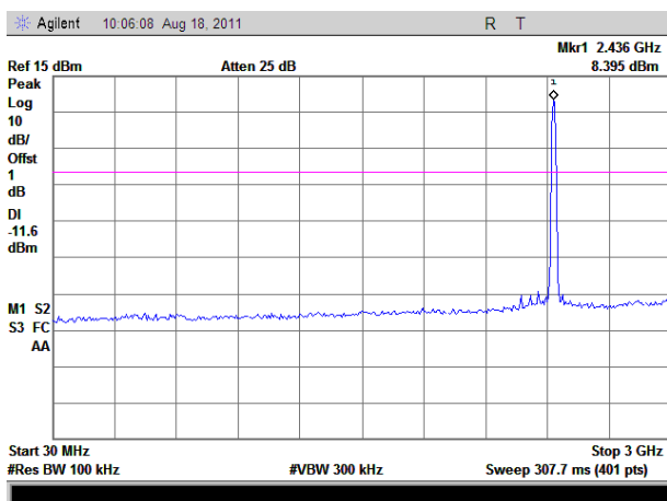
(Plot B.3: Channel = 6, 30MHz to 3GHz)
