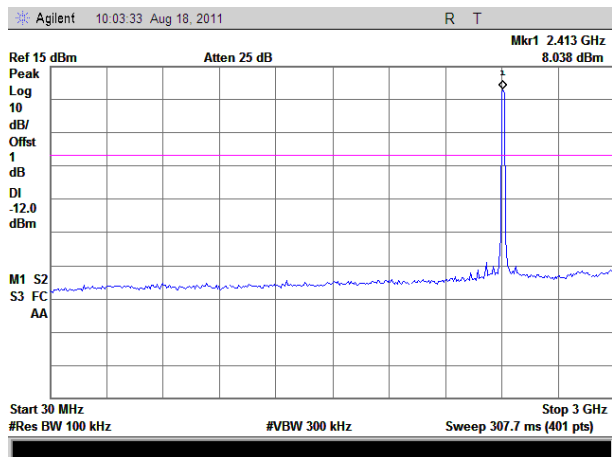
(Plot A.3: Channel = 1, 30MHz to 3GHz)
