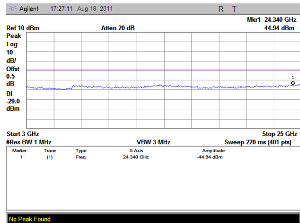
(Plot A.4: Channel = 3, 3GHz to 25GHz)
