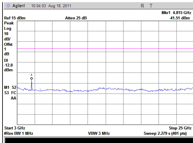
(Plot A.4: Channel = 1, 3GHz to 25GHz)
