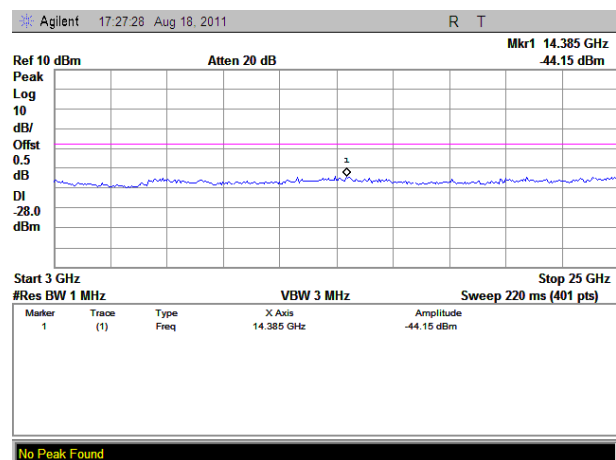
(Plot B.4: Channel = 6, 3GHz to 25GHz)
