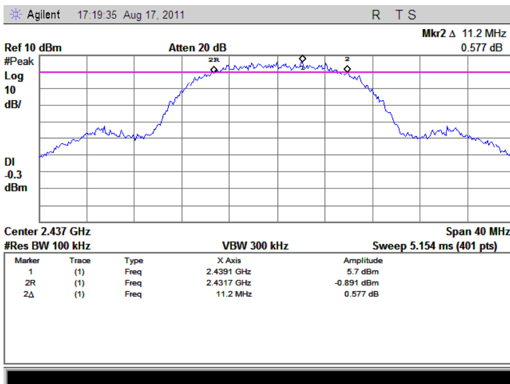
(Plot B1: Channel 6: 2437MHz @ 802.11b)
