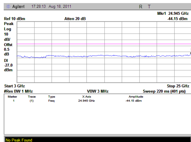
(Plot C.4: Channel = 9, 3GHz to 25GHz)
