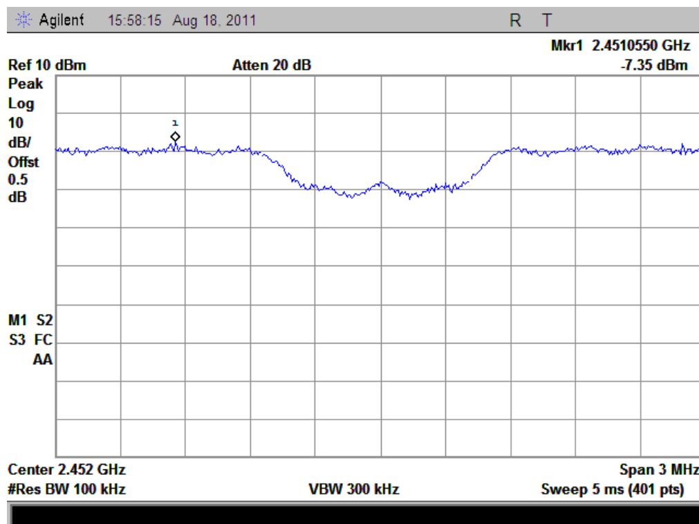
(Plot L.1: Channel = 9 @ 802.11n)
