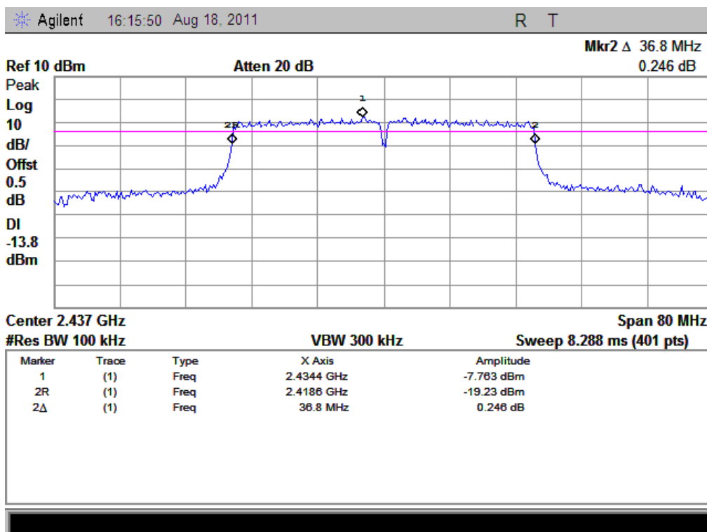
(Plot K1: Channel 6: 2437MHz @ 802.11n)
