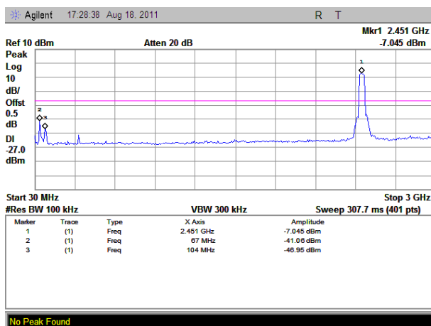
(Plot C.3: Channel = 9, 30MHz to 3GHz)
