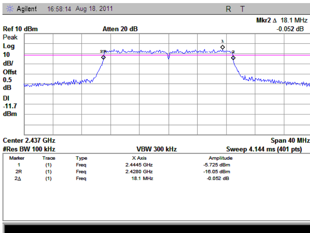
(Plot H1: Channel 6: 2437MHz @ 802.11n)
