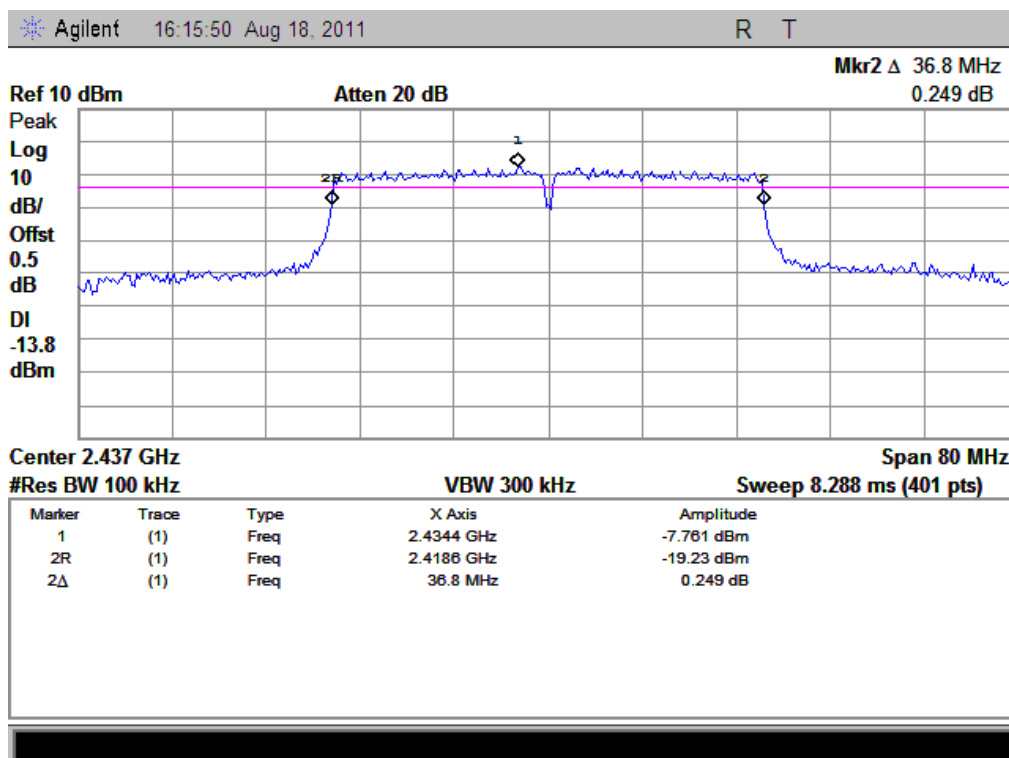
(Plot K: Channel 3: 2437MHz @ 802.11n)
