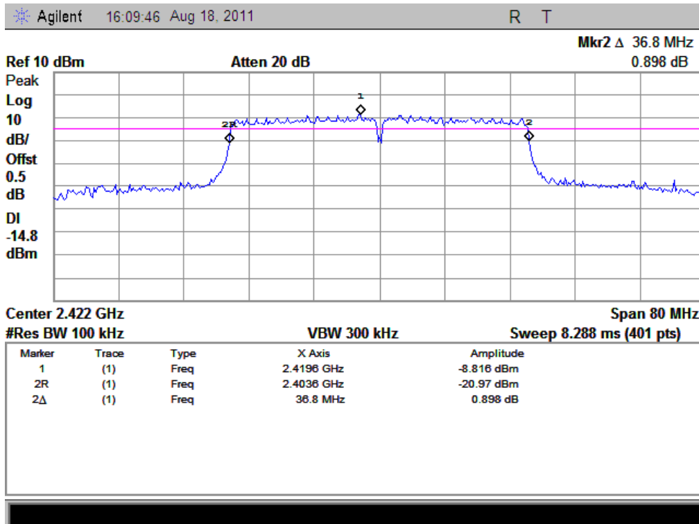
(Plot J1: Channel 3: 2422MHz @ 802.11n)
