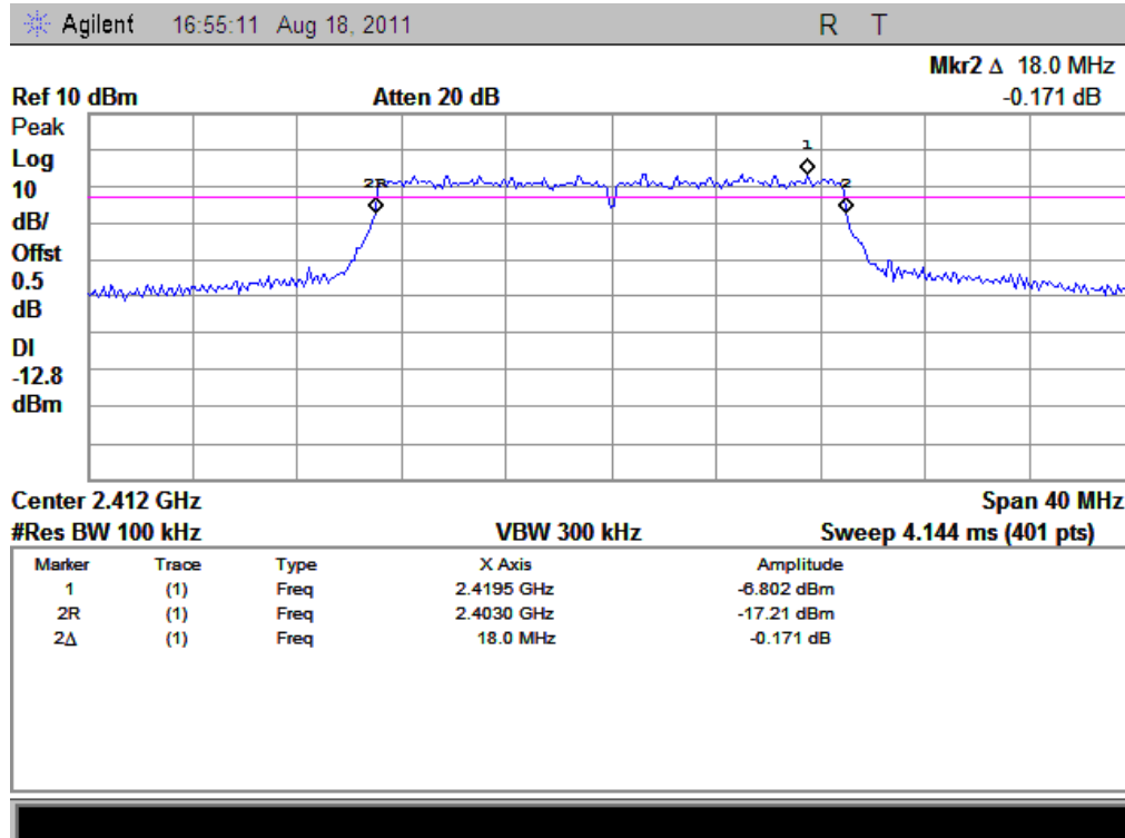
(Plot G: Channel 1: 2412MHz @ 802.11n)
