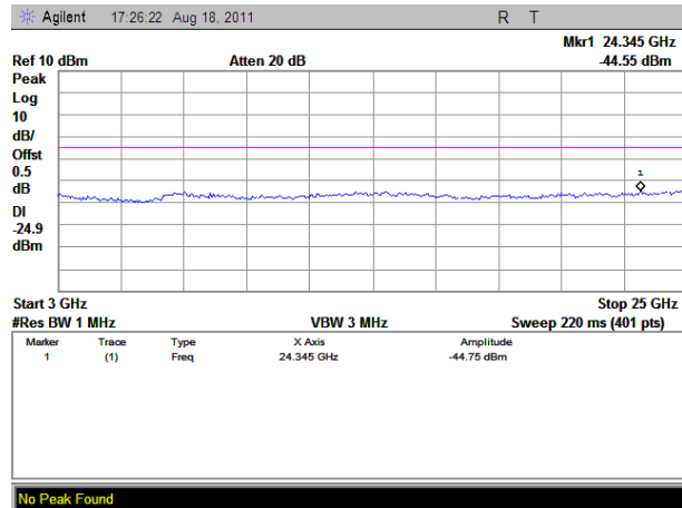
(Plot C.4: Channel = 11, 3GHz to 25GHz)
