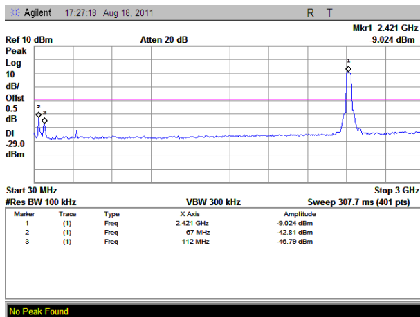
(Plot A.3: Channel = 3, 30MHz to 3GHz)
