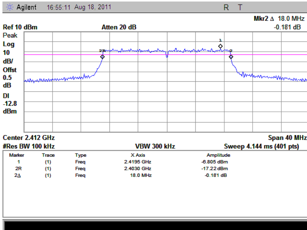
(Plot G1: Channel 1: 2412MHz @ 802.11n)
