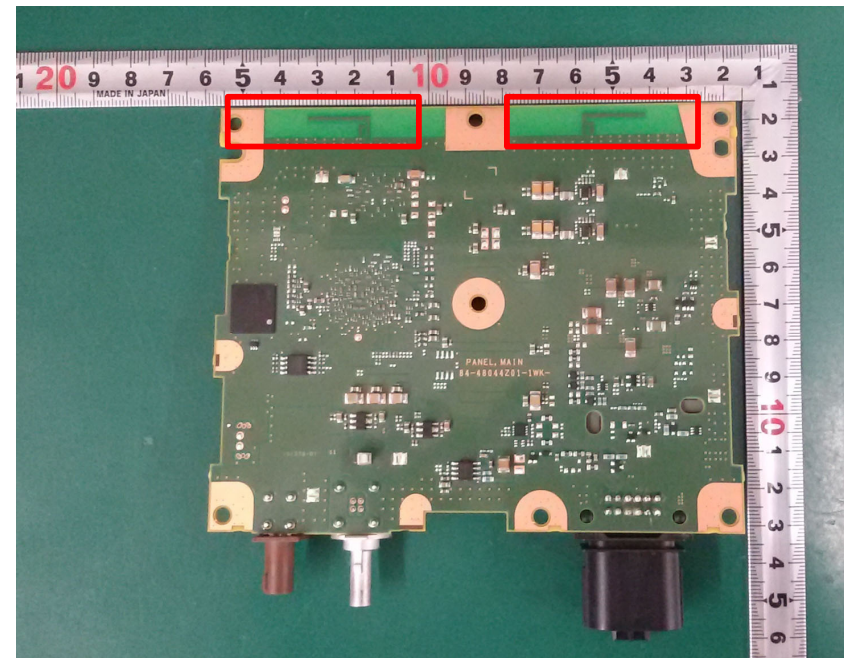
2.4GHz_BT ANT
