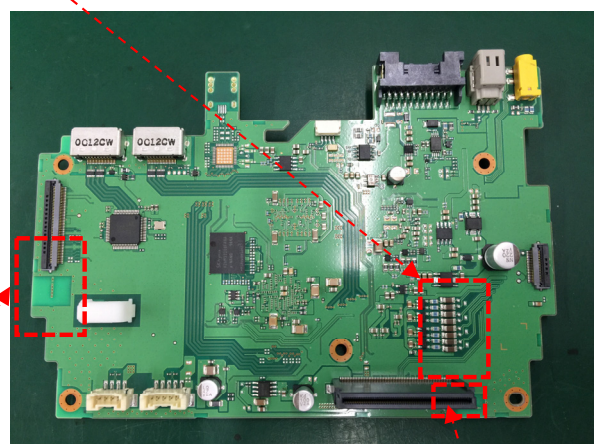
BT ANTENNA
