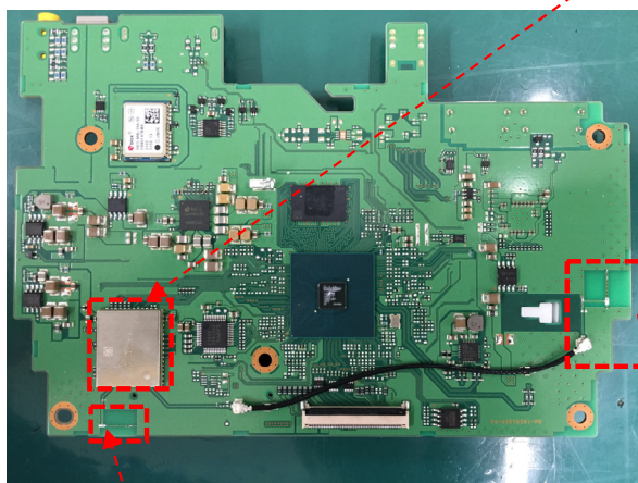
BT ANTENNA
