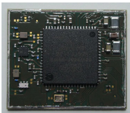
BT_WiFi Module Internal photo
