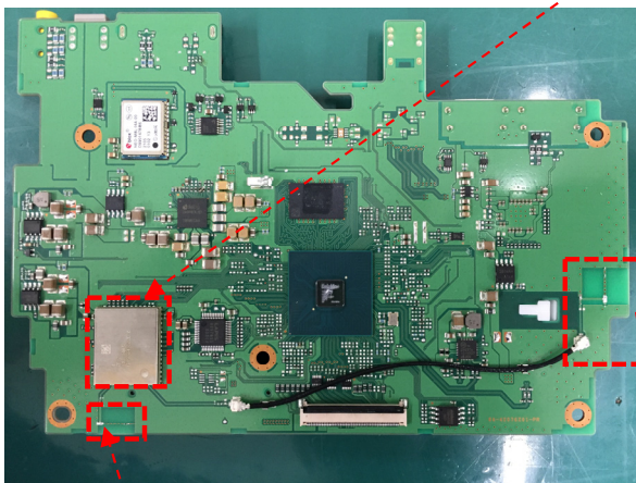
BT ANTENNA
