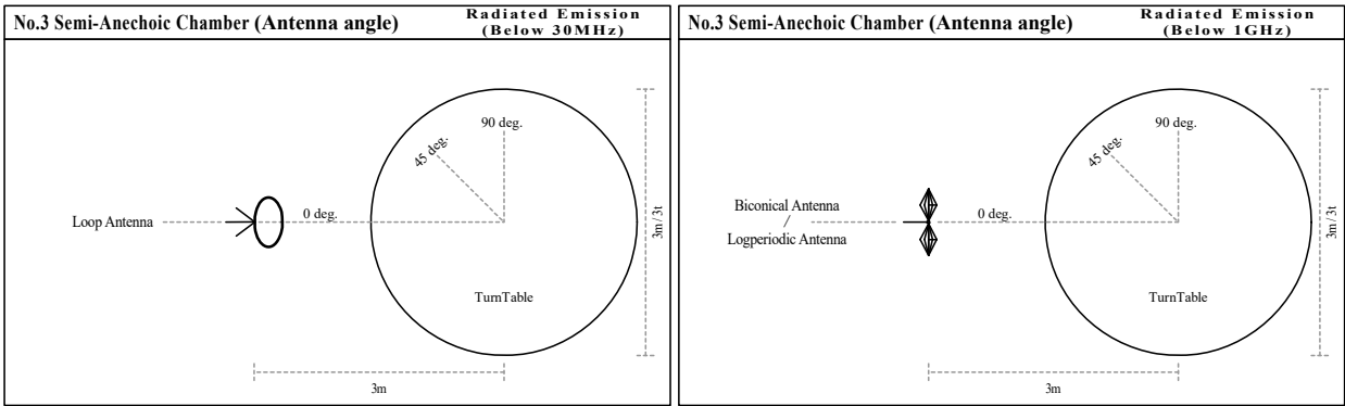
Figure 2. Antenna angle
