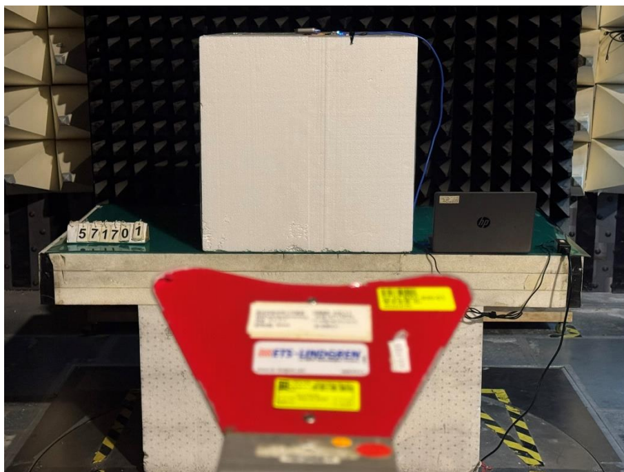
06. RADIATED BAND EDGE Rear View(1GHz above)
