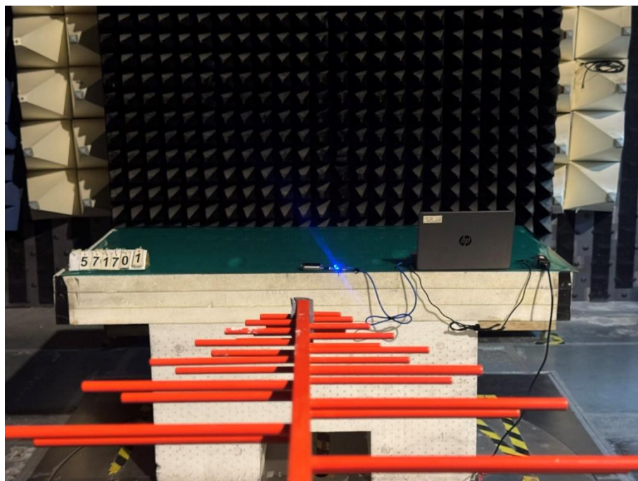
04. RADIATED BAND EDGE Rear View(1GHz below)
