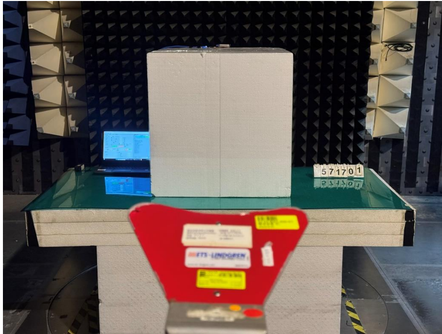
05. RADIATED BAND EDGE Front View(1GHz above)
