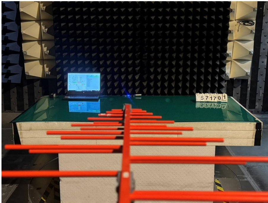
03. RADIATED BAND EDGE Front View(1GHz below)
