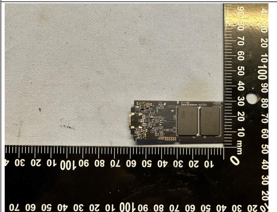
02. Front view of PCB 1
