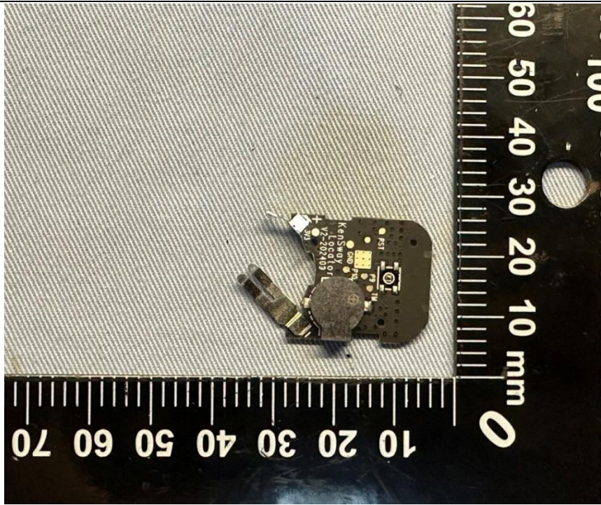
05. Rear view of PCB 2
