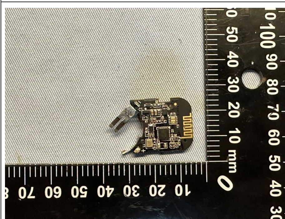
04. Front view of PCB 2
