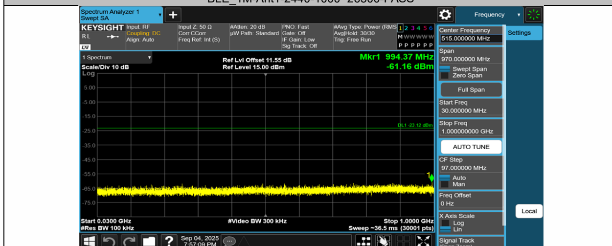
BLE_1M-Ant1-2480-30~1000-PASS
