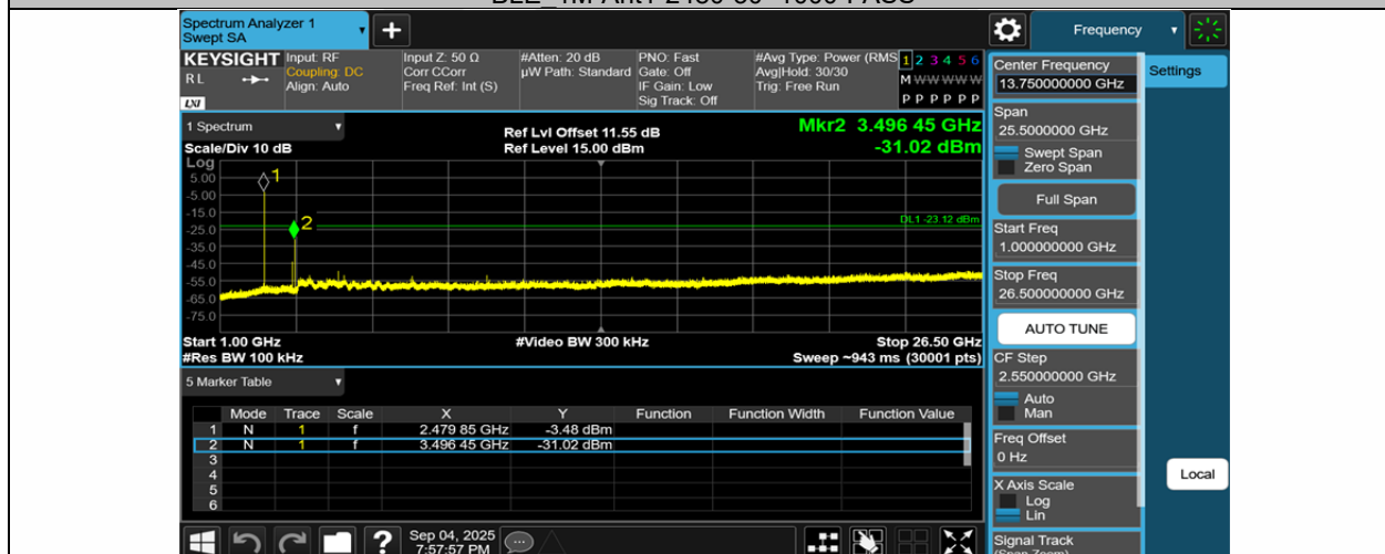
BLE_1M-Ant1-2480-1000~26500-PASS
