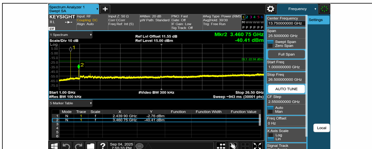
BLE_1M-Ant1-2440-1000~26500-PASS
