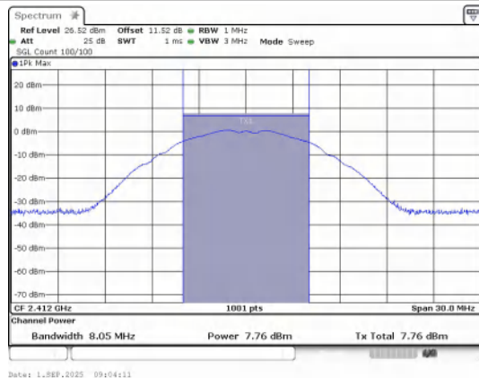
Conducted Output Power IEEE 802.11b_Channel 1_Antenna 0
