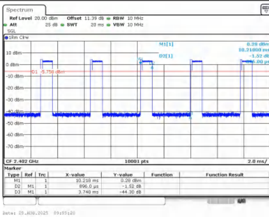
8DPSK(3-DH5)_Channel 0
